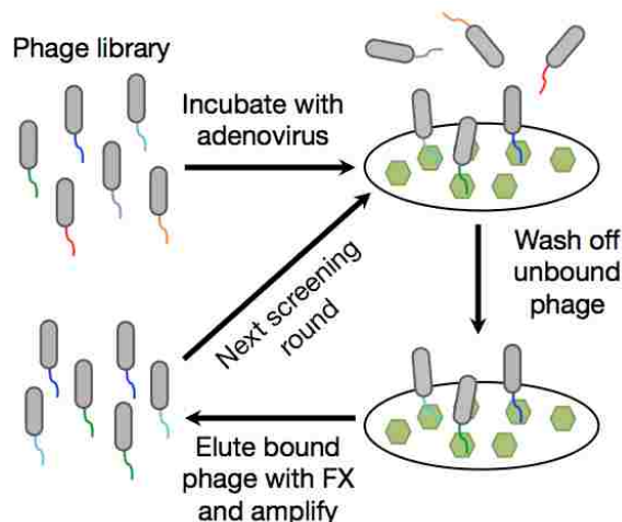
Figure 6.1 Phage panning strategy using competitive displacement with FX protein to elute adenovirus-binding phage.
