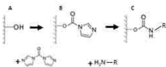
Figure 3-1. Carbonyl diimidazole immobilization reaction
