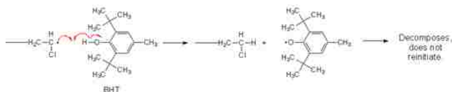
Figure 2-5 BHT inhibition of polymerization by scavenging of free radicals
