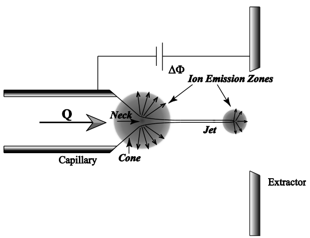
Figure 1.1. Simplified diagram of an electro spray capillary emitter and extractor assembly.
