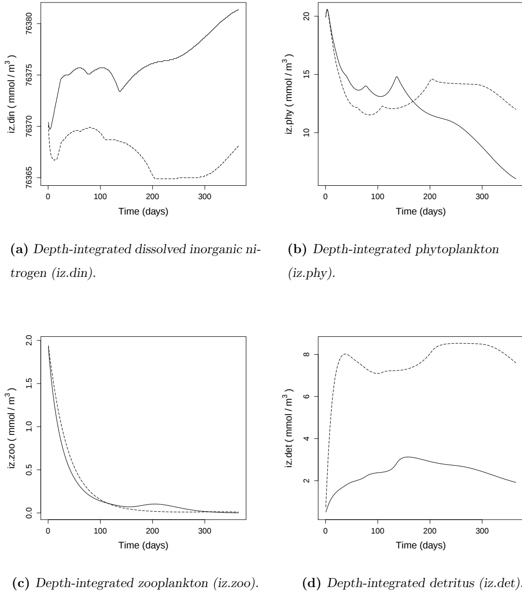
Figure 2.3: Time series outputs for the depth-integrated versions of the four main tracers. The input points were the two ‘default’ points, one for each simulator. The solid line corresponds to the HadOCC run and the dashed line to the OG99NPZD run.
