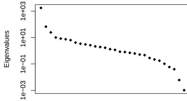
Figure 6.8: Eigenvalues of \Sigma_{\text{OG}}^{-1}\Sigma_{\text{HAD}} (log-scale)
