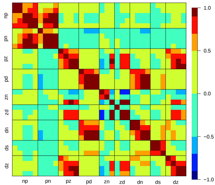
(b) HadOCC
