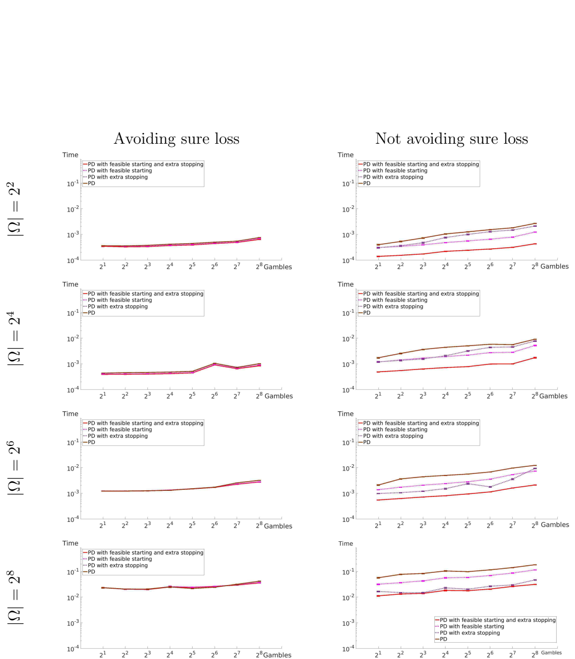
Figure 9.10: Comparison plots of the average computational time for different improved primal-dual methods (PD) for solving (P3) and (D5) where we fix the number of outcomes and vary the number of desirable gambles. The labels indicate different primal-dual methods.
