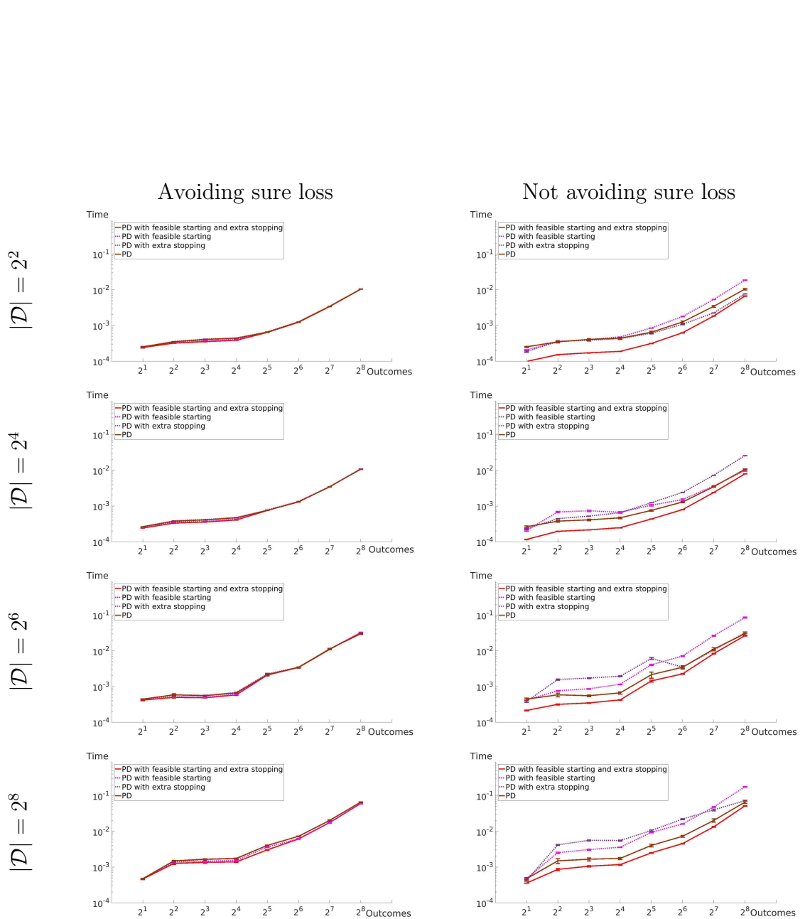
Figure 9.8: Comparison plots of the average computational time for different improved primal-dual methods (PD) for solving (P3) and (D5) where we fix the number of desirable gambles and vary the number of outcomes. The labels indicate different improved primal-dual methods.
