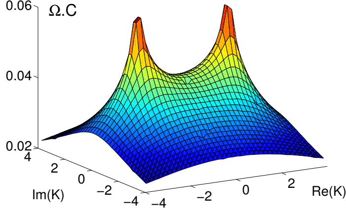
Figure 4.5: Surface plot of the conformal factor. Peaks are at K = \pm 2C .
