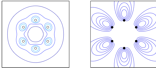
Figure 3.13: D_6 -symmetric \mathbf{k} = (2, 1) periodic monopole with spectral curve w^3 - \zeta^2 w^2 - 1 = 0 . On the left is plotted the energy density and on the right the discriminant of \hat{\Phi} .
