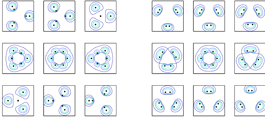
Figure 6.1: Cross section of energy density for two one-parameter families with b_1 = 0 . Left: b_0 \in \mathbb{R} with b_0 = -4, -3, \dots, 4 . The relevant symmetries are i, ii, iv and vi in the list of section 6.1. Right: b_0 \in i\mathbb{R} with -ib_0 = -4, -3, \dots, 4 , with symmetries i, ii, v and vii. In both cases these define the dihedral symmetry group D_3 .
