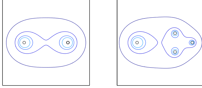
Figure 3.10: Deformations of the \mathbf{k} = (1, 1) monopole with \mathbf{v}_2 = 0 . On the left are contours of energy density for \mu_1 e^{\mathbf{v}_1} = 1 . On the right, for \mu_1 e^{\mathbf{v}_1} = 1.2 . For these examples, the discriminant pairs up the spectral points on the horizontal axis. The line of zero discriminant joining the other two points is found to wrap around the left hand spectral point.
