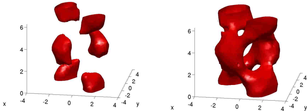
Figure 5.5: Energy density isosurfaces for C = 4 , W = i . On the left we see the constituent structure, and on the right the twisted chain. The symmetry group can be equivalently described as D_{2h} \times \mathbb{Z}_2 or D_{2d} \times \mathbb{Z}_2 . The eight axes of rotational symmetry are (x = \pm y, z = 0) , (x = \pm y, z = \beta/2) for D_{2h} symmetry, and (x = 0, z = \pm\beta/4) , (y = 0, z = \pm\beta/4) for D_{2d} symmetry. Note also the similarity to the Skyrminion chain configurations obtained in [HW08].
