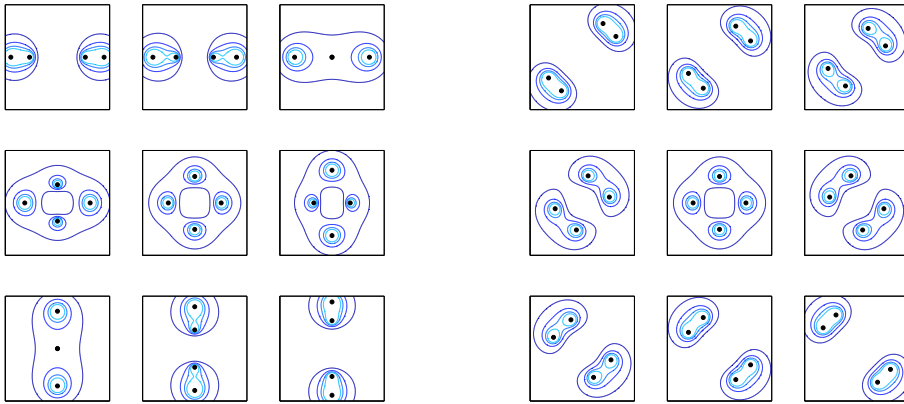
Figure 3.3: Energy density contour plots for charge k = 2 within the spectral approximation. Left: geodesic with K \in \mathbb{R} (to be read from left to right and top to bottom). Right: geodesic with K \in i\mathbb{R} . The central symmetric configurations have K = 0 , while those with just two energy peaks have K/C = \pm 2 . It is noteworthy that the axial symmetry of the ‘doughnut’ charge 2 monopole in \mathbb{R}^3 [War81] is replaced by a discrete dihedral ( D_4 ) symmetry. Note how the constituents themselves (indicated by black dots) as well as the monopoles as a whole undergo 90^\circ scattering. The spacing between snapshots is taken relative to the metric defined in section 3.3.
