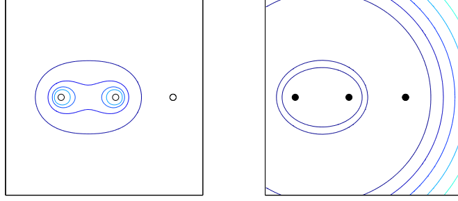
Figure 3.9: Deformations of the \mathbf{k} = (1, 1) monopole by changing \mathbf{v}_2 away from zero. Here \mathbf{v}_2 = 1.2 and \mu_2 = 0 . On the left is plotted the energy density and on the right the discriminant of \hat{\Phi} . There is no energy density associated with the coincident spectral points on the right. The discriminant vanishes on a line joining the spectral points on the left, and on a circle passing through the double spectral point and surrounding the other two.
