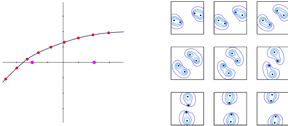
Figure 3.6: Geodesic for initial conditions K/C = 5 + 2i , \dot{K}/C = -0.042 with step size 0.03. Tick marks are at every 950 timesteps. In this case the fundamental monopoles retain their separate identities.
