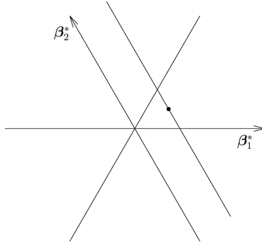
Figure 3.12: Deformation of the subleading term. Starting from the shaded point we deform parallel to \beta_2^* .
