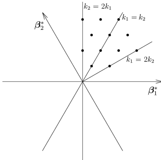
Figure 2.1: Root diagram for SU(3) showing magnetic weights (k_1, k_2) allowed by (2.2).
