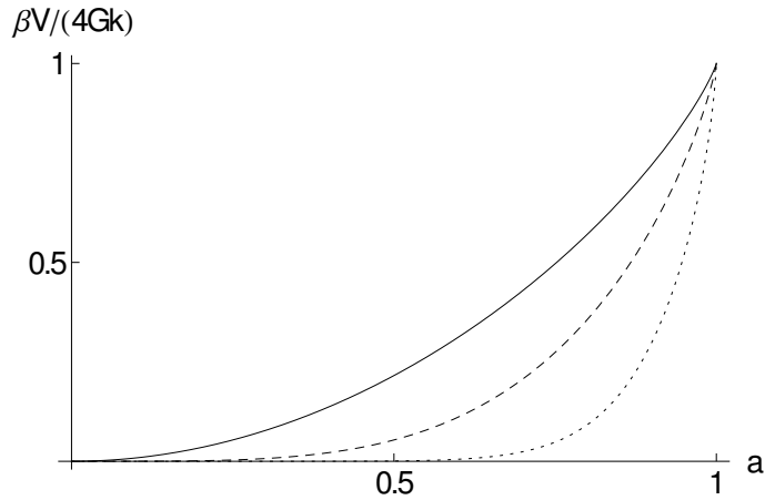
Figure 3.2: Normalised energy per unit charge enclosed in a period cylinder of radius aC^{1/k} for various values of the charge k . Solid line: k = 1 , dashed: k = 2 , dotted: k = 10 . The energy density is increasingly located on a shell of radius \rho = C^{1/k} .
