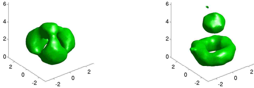
Figure 6.4: Energy density of a charge 3 periodic monopole with C = 1 taken over a single period. Left: approximately tetrahedral configuration with W = 2 + \sqrt{3} ( K = 4 ). Right: when W = i , clusters of charge 1 and 2 are visible. The symmetry groups are C_{3v} and D_{3d} , respectively.
