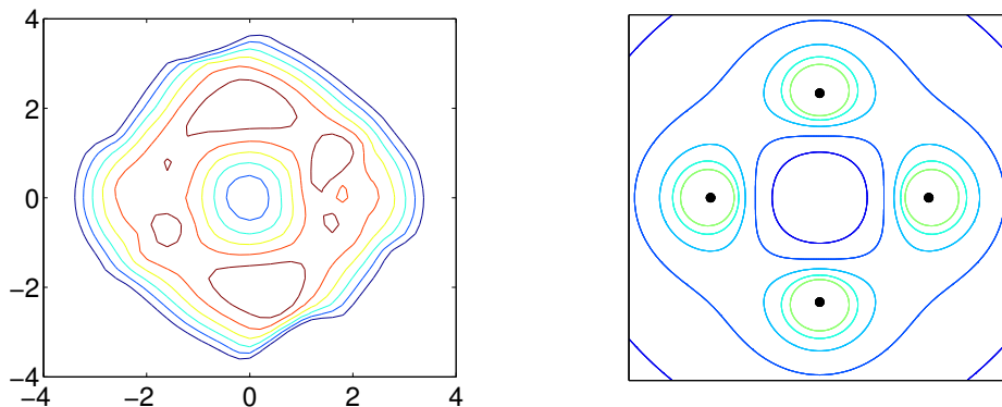
Figure 5.9: Left: energy density integrated over a period for C = 4 , W = i . Unlike in figure 5.5, the energy peaks here are at the locations expected from the spectral approximation (right). Note that this comparison requires a rescaling of the x and y coordinates by a factor of \sqrt{C} .
