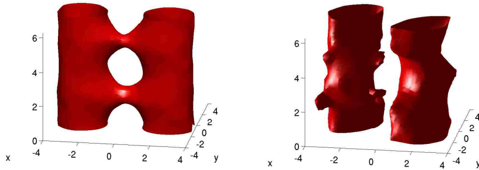
Figure 5.7: Scattering for C = 4 on the |W| = 1 geodesic. Left: W = 1 with symmetry group D_{2h} \times \mathbb{Z}_2 ; right: W = e^{i\pi/3} with symmetry group D_{2h} . The W = i configuration is shown in figure 5.5.
