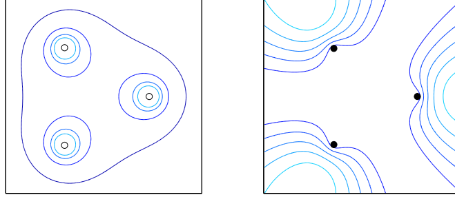
Figure 3.11: D_3 -symmetric \mathbf{k} = (2, 1) periodic monopole with spectral curve w^3 - \zeta^2 w^2 + 2\zeta w - 1 = 0 . Energy density on the left and the discriminant of \hat{\Phi} on the right.
