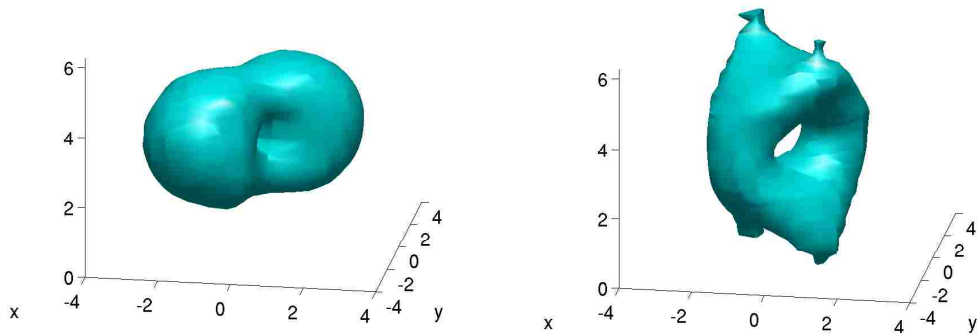
Figure 5.6: Two points on the W = i\mathbb{R} geodesic with C = 2 , displaying D_{2h} symmetry. Left: W = 2i , right: W = 1.125i . As well as illustrating the scattering process, these energy density plots show how there is a transition between the C = 1 case, where the energy is peaked in two regions near the z -axis, and the C = 4 case, in which the energy is peaked away from the z -axis. The ‘four pronged’ structures of figure 5.2 can be visualised as splitting the right hand structure above along z = \pi .
