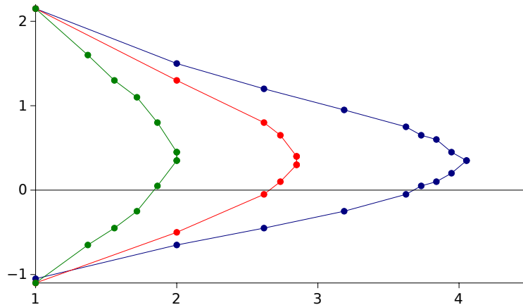
Figure 6.5: Motion of the zero-antzero pair along the z -axis (with 0 corresponding to z = \beta/3 , and \beta = 2\pi ) as a function of W for various values of C : C = 1 in blue (rightmost curve), C = 2 in red (middle) and C = 5 in green (left). For small C , the value of W at which the lower zero (the antzero) is centered at z = \beta/3 appears to coincide with the monopole configuration closest to tetrahedral symmetry (figure 6.6).
