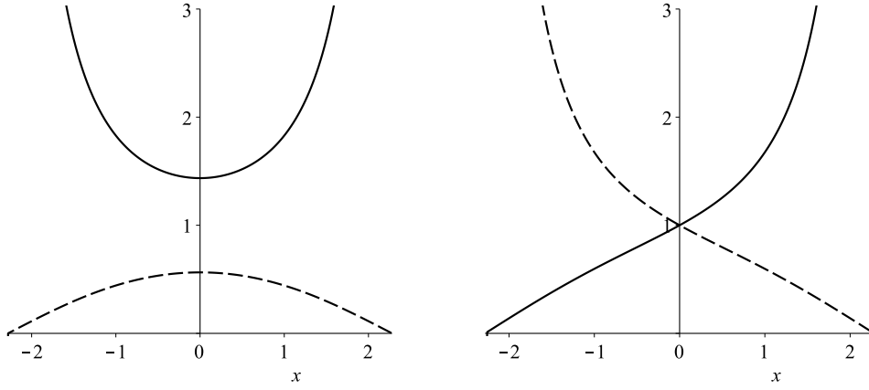
Figure 5.4: Left: (f_1 + f_2)/a (solid) and (f_1 - f_2)/a (dashed) for k = 0.9 plotted against x = ar , for f_1^2 > f_2^2 > f_3^2 . Right: (f_1 + f_2)/\sqrt{2K} (solid) and (f_1 - f_2)/\sqrt{2K} (dashed) against x = \sqrt{2K}r , for f_1^2 > f_3^2 > f_2^2 .
