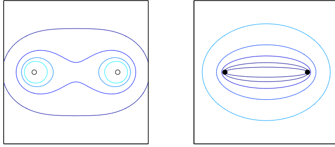
Figure 3.1: An SU(2) periodic monopole. On the left is a contour plot of the energy density (3.10) and on the right of \log(\text{disc}(\hat{\Phi}) + 0.001) . The discriminant vanishes on a line joining the spectral points, whose locations are indicated by black dots on the right hand diagram. Note the loss of axial symmetry and the appearance of constituents, which coincide when the monopole size |C| = 0 (when \arg(C) can have no effect).
