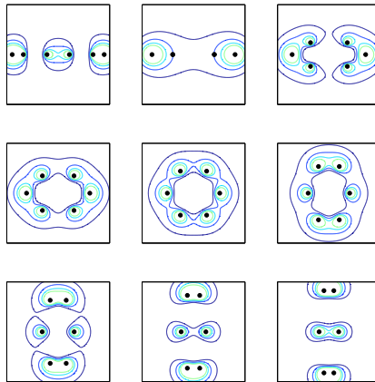
Figure 6.2: Energy density for b_1 \in \mathbb{R} , b_0 = 0 , with b_1 = -4, -3, \dots, 4 . Unlike the symmetries in figure 6.1, this family does not have a charge 2 analogue, and in fact the Nahm data is only known for the special case b_1 = -3 , b_0 = 0 (top row, central panel). This configuration is in fact a charge 1 chain with period \beta/3 and is described in section 6.3.1. The symmetry group is D_2 , described by i, iii, iv and vii in the list above.
