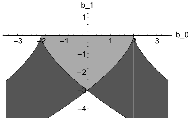
Figure 6.3: Regions of the moduli space for which a charge 3 monopole contains a single cluster (light grey), two clusters (dark grey) and three clusters (white). The lines on which (6.3) holds are shown in black.
