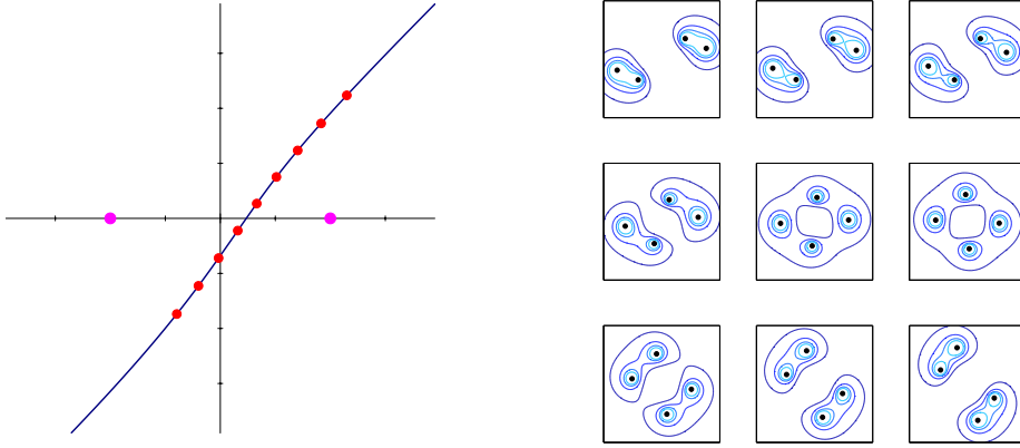
Figure 3.5: Geodesic for initial condition K/C = 5(1+i) , \dot{K}/C = -0.03(1+i) with step size 0.03. The left hand plot displays the geodesic on the K -plane (with shaded circles at K/C = \pm 2 ). Tick marks every 722 timesteps indicate the positions of the energy density snapshots displayed to the right.
