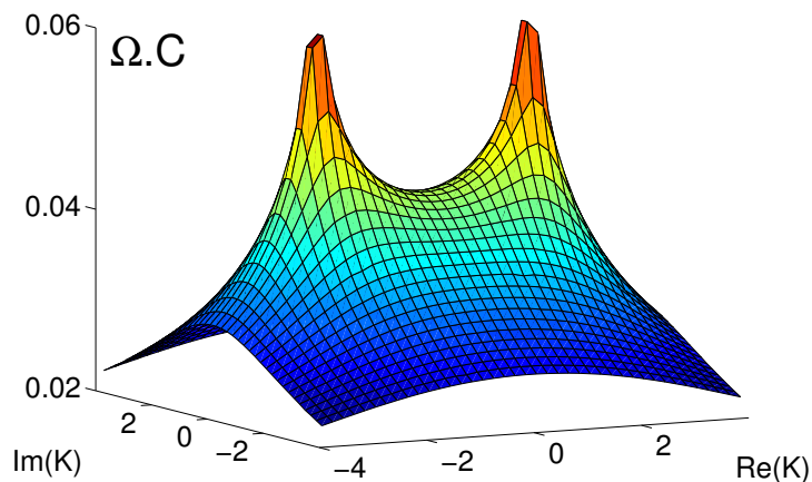
Figure 3.4: Surface plot of the conformal factor, computed from (3.24), for the relative reduced moduli space in the limit of large monopole size to period ratio, with \beta = 2\pi . The infinite peaks (3.26) are at K/C = \pm 2 .
