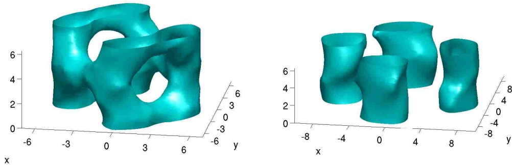
Figure 5.8: Left: C = 16 , W = i , right: C = 36 , W = i . Note how we approach the z -independent result of the spectral approximation (figure 3.3, middle panel).
