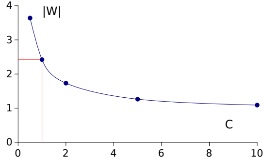
Figure 5.1: |W| against C , showing how the value of |W| at which the monopole Higgs zeros coincide in the ‘zeros apart’ configuration depends on C , both for W \in \mathbb{R} and W \in i\mathbb{R} . For ‘zeros together’, the monopole zeros always coincide when K = 0 .
