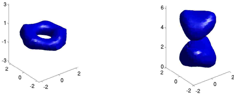
Figure 5.2: Energy density for a charge 2 monopole chain (taken over one period) in the ‘zeros together’ (left) and ‘zeros apart’ (right) configurations with \beta = 2\pi , C = 1 and W = i . In the notation of section 4.1.2 these configurations have symmetry groups D_{4h} and D_{2d} \times \mathbb{Z}_2 .
