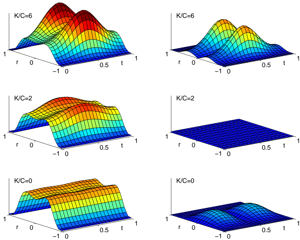
Figure 4.1: Lumps in |B| for various values of K in the ‘zeros together’ solution (left) and the ‘zeros apart’ solution (right) for C = 1 and \beta = 2\pi , using the same vertical scale throughout. The positions of the lumps should be compared with the positions of the zeros of \det(\Phi) , as indicated in figures 3.7 and 3.8. It should also be noted that the lumps are of different sign in each case.
