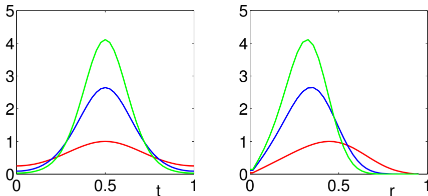
Figure 4.2: Profiles through the maxima of |B| in the t and r directions for various values of C , with K/C = 6 and \beta = 2\pi in the ‘zeros apart’ configuration. The height of the C = 1 peak (red) is used to normalise those for C = 5 (blue) and C = 10 (green). Notice how the peaks get narrower as C is increased. The r positions of the maxima (approximately 0.42, 0.33 and 0.30, respectively) approach the position of the zero of \det(\Phi) , at r = \beta^{-1} \cosh^{-1}(K/2C) \approx 0.28 .
