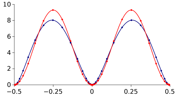
Figure 4.4: Effective potential for the kinks in figure 4.3 (blue) compared with the sine-Gordon potential (4.11) of the same energy (red), which fixes \lambda \approx 9.3 .
