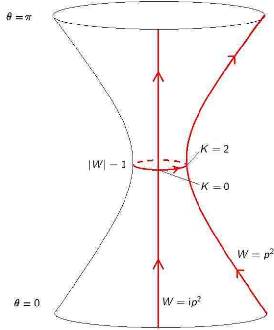
Figure 4.8: Sketch of the ‘double trumpet’ showing the geodesics with W \in \mathbb{R} , W \in i\mathbb{R} and |W| = 1 identified in section 4.1.2.
