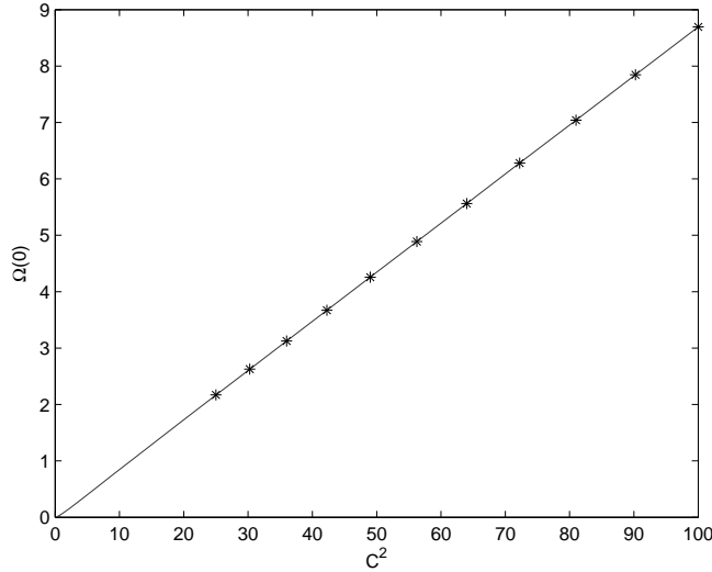
Figure 4.6: g_{K_W \overline{K_W}}(K = 0) against C_W^2 = C/2 for numerical solutions with \beta = 2\pi , with a straight line fit of gradient 0.0870 (the analytical gradient expected from (4.23, 4.24) is g(0) \approx 0.08708 ). The ‘large C limit’ appears to be a good approximation for C \gtrsim 50 . (Note the scaling with C arises from combining the conformal factor (4.22) with the rescaled K coordinates.) [Unpublished figure due to Ward.]
