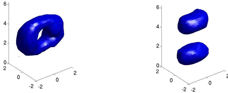
Figure 5.3: Energy density for a charge 2 monopole chain in the ‘zeros apart’ configuration with C = 1 and W = 2.43 (left) and W = 1 (right). These configurations show the symmetries D_{2h} and D_{2h} \times \mathbb{Z}_2 .
