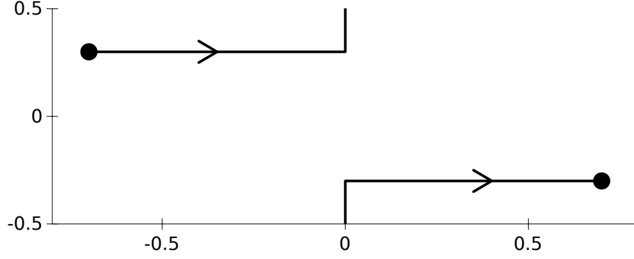
Figure 4.7: Contour on the Hitchin cylinder used to parallel propagate f_- from s_- (the left dot) to s_+ on the right. Circling the cylinder in the opposite direction modifies L to L \approx h_0(\pi - \varphi)/\beta .
