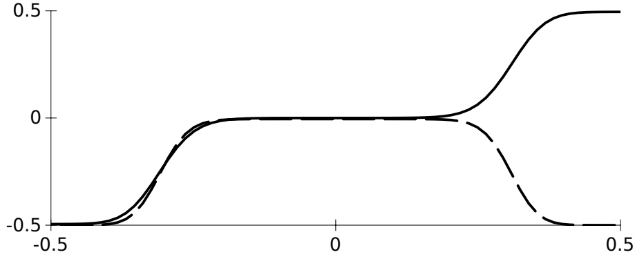
Figure 4.3: 2\gamma/\pi as a function of r for the ‘zeros together’ solution (solid line) and the ‘zeros apart’ solution (dashed line), in both cases with K/C = 7 , C = 200 and \beta = 2\pi .
