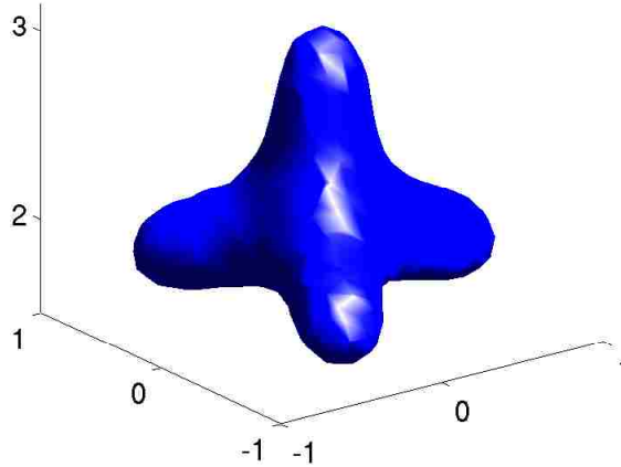
Figure 6.6: A contour of \text{tr}(\hat{\Phi}^2) for the C = 1 , W = 2 + \sqrt{3} ( K = 4 ) charge 3 solution of type \ell = 1 . This shows the Higgs field is close to zero at the centre of the tetrahedron, although the energy density is not peaked there (see figure 6.4, but note the change of scale).
