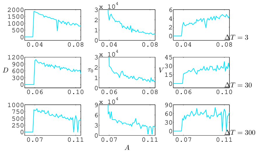
Figure 3.8: Polaron displacement, D , lifetime, \tau_0 , and displacement per pulse, V , as functions of time-span \Delta T and amplitude A of time-periodic pulses. 1000 units of \tau equals 3.2 ps.
