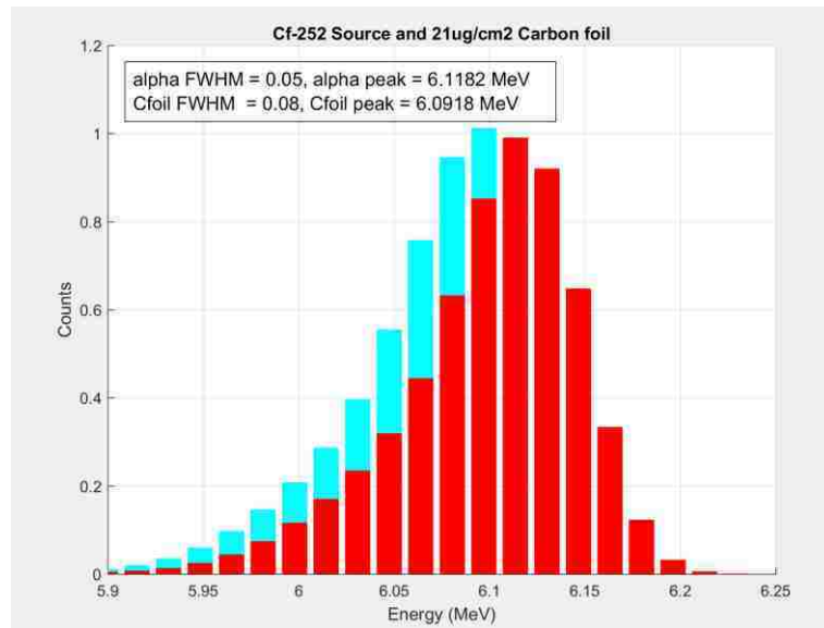
Figure 55: ^{252}\text{Cf} 6.118 MeV alpha peak (red) with a 21\text{ }\mu\text{g}/\text{cm}^2 alpha spectrum (blue).
