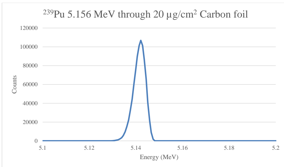
Figure 33: MCNP experiment simulation.
