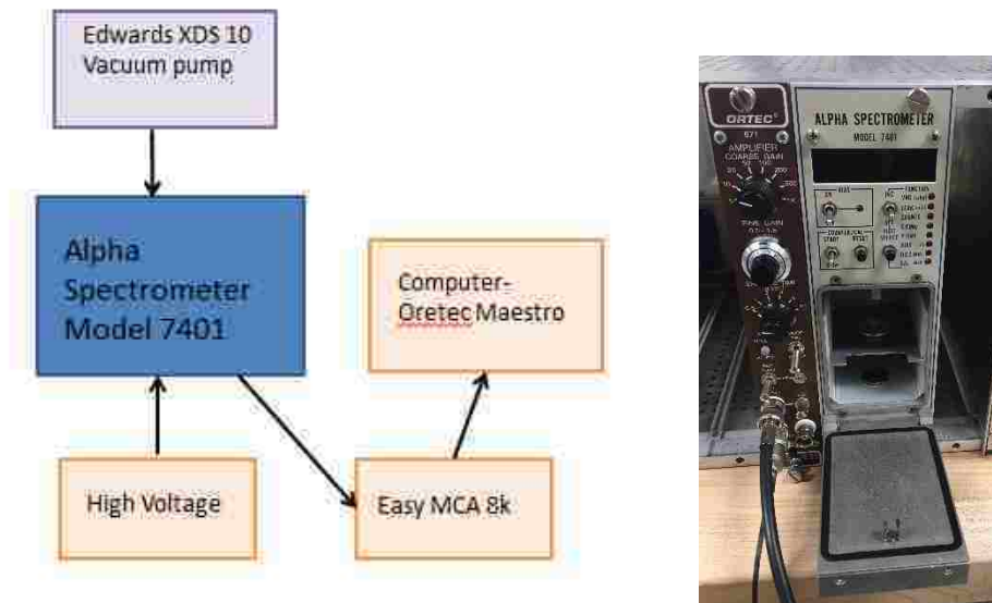
Figure 45: Block diagram of alpha energy loss experiment (left) and Alpha Spectrometer Model 7401(right).
