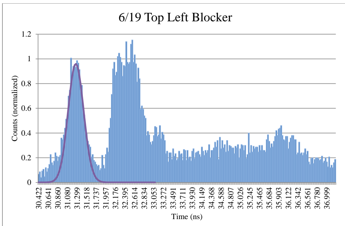
Figure 30: ^{239}\text{Pu} source and Top Left Blocker TOF spectrum.
