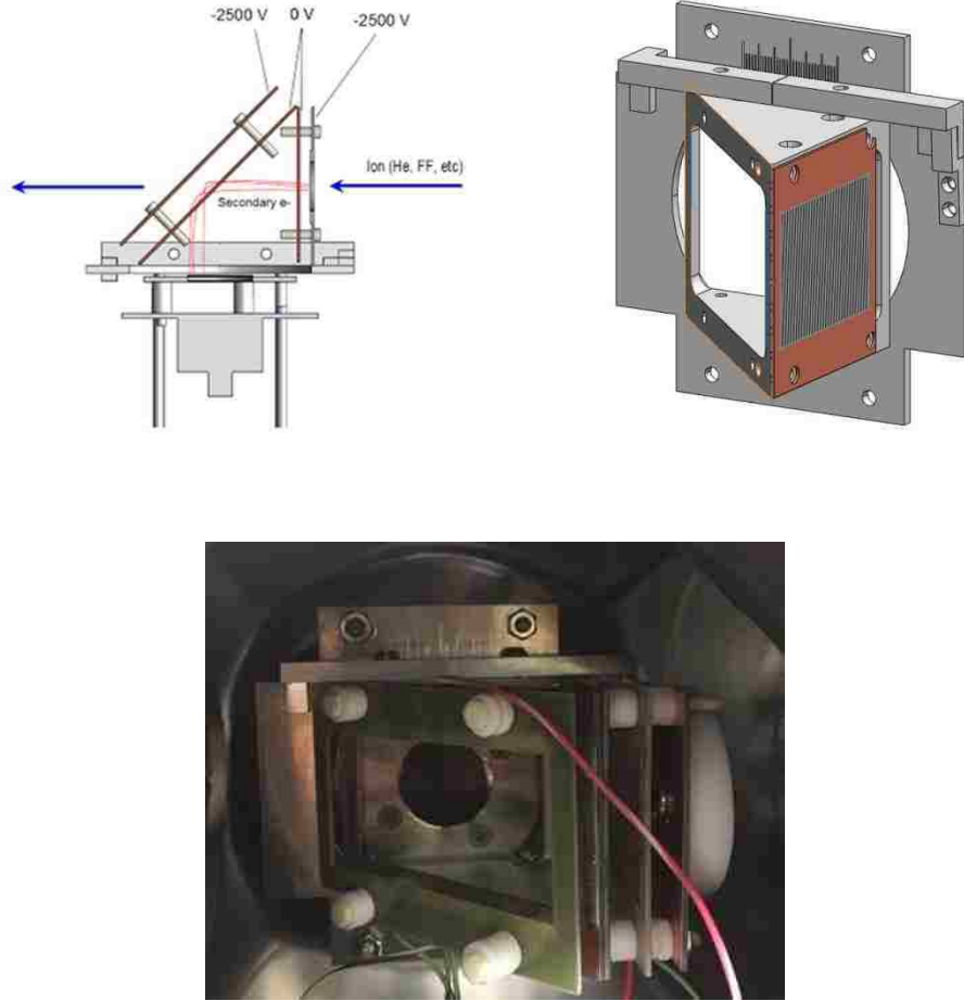
Figure 5: TOF timing module SolidWorks models (Top) and a photo (Bottom).
