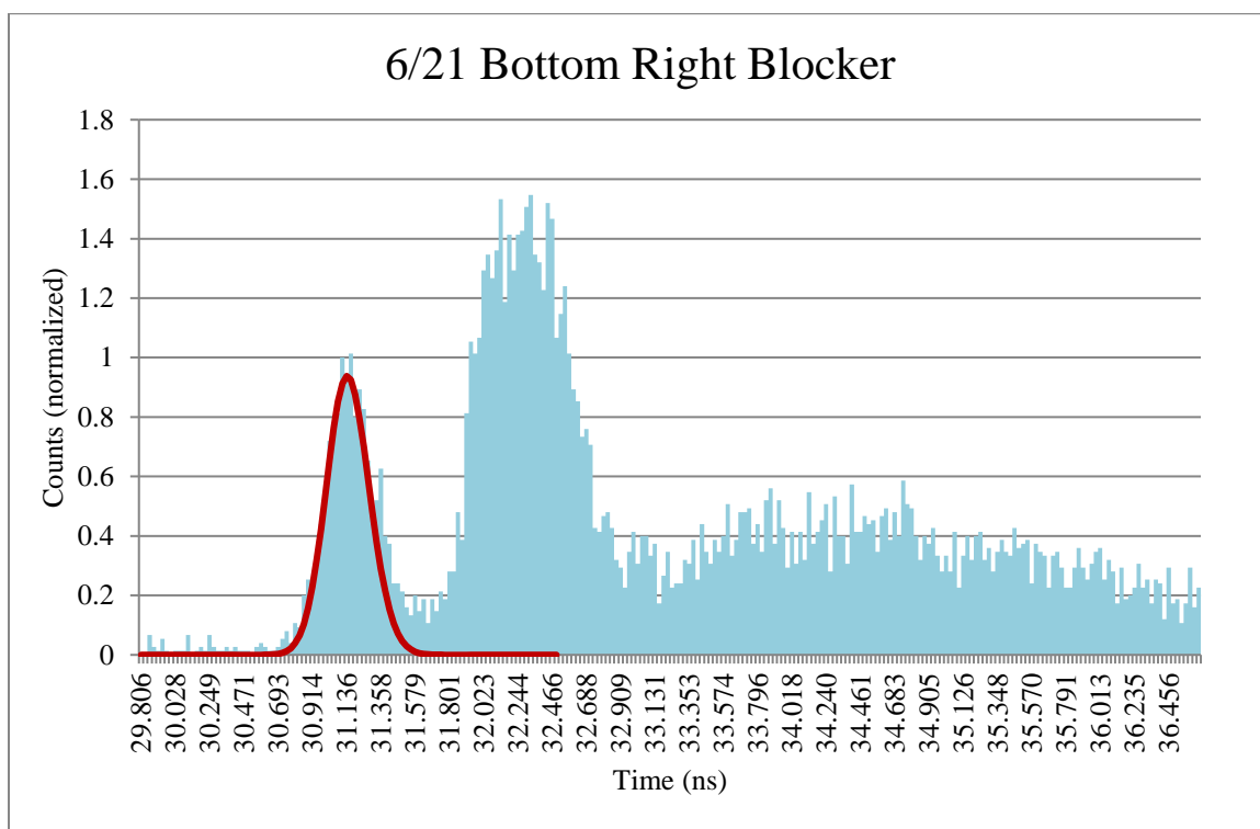
Figure 31: ^{239}\text{Pu} source and Bottom Right Blocker TOF spectrum.
