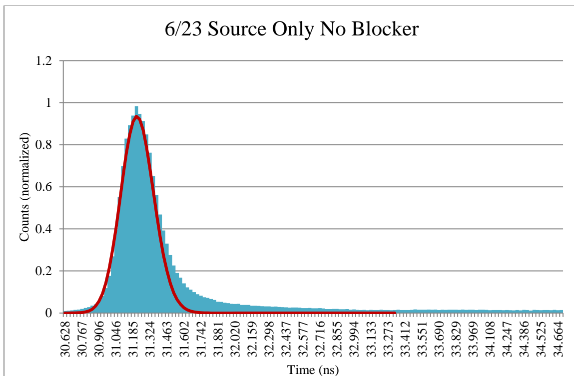
Figure 28: ^{239}\text{Pu} source and No blocker of TOF spectrum.
