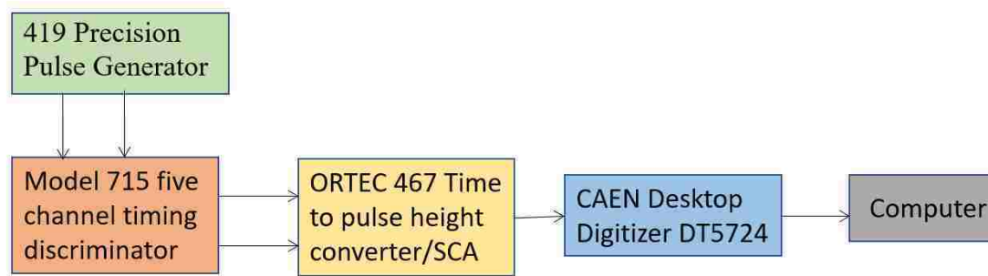
Figure 18: Block diagram of calibration with signal split before discriminator.
