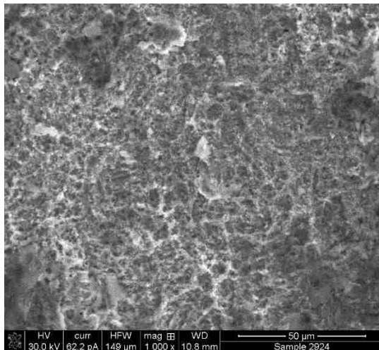
Figure 58. Series 5.1 SEM image after descaling with ammonium persulfate
