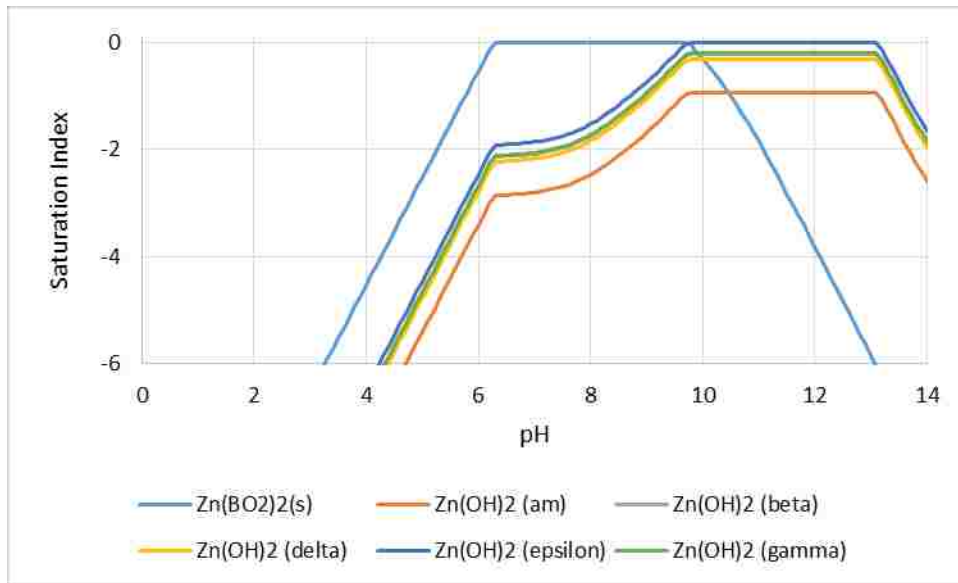
Figure 4. Saturation indices for unbuffered 100 mg/L initial zinc
