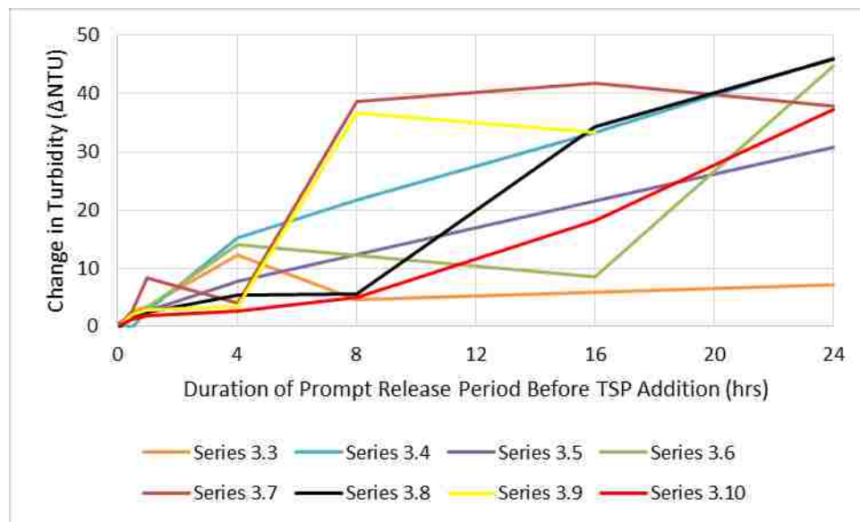
Figure 46. Theme 3 turbidity measurements
