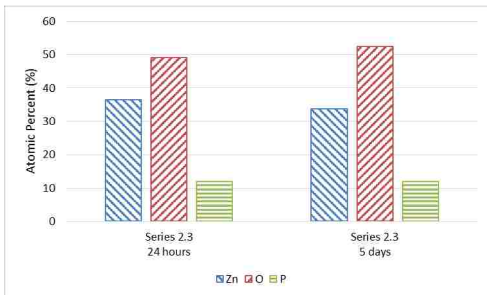
Figure 36. Series 2.3 (pure zinc) EDS spectral results
