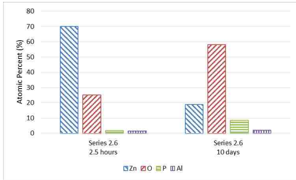
Figure 37. Series 2.6 (galvanized steel) EDS spectral results
