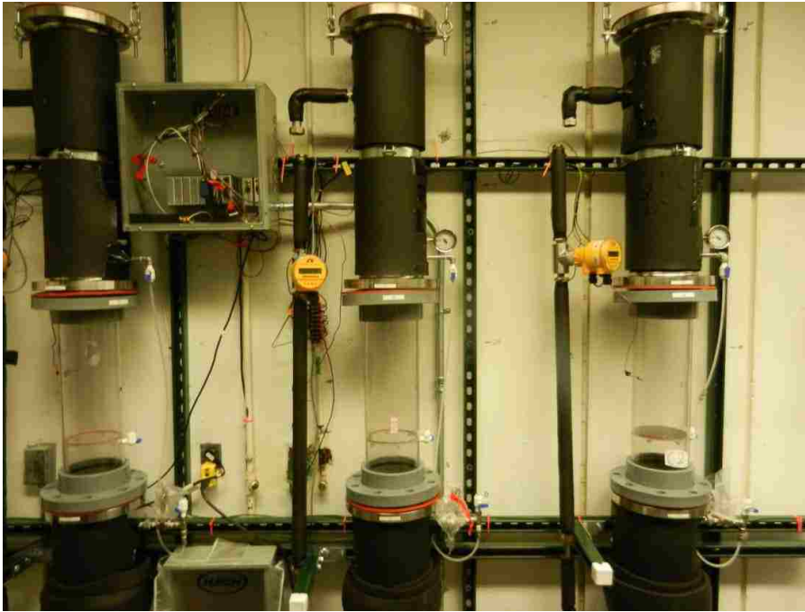
Figure 9. CHLE vertical strainer head loss columns [19]
