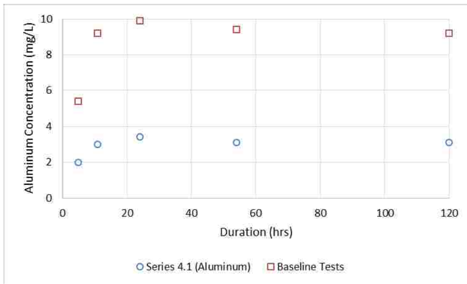
Figure 55. Series 4.1 aluminum release
