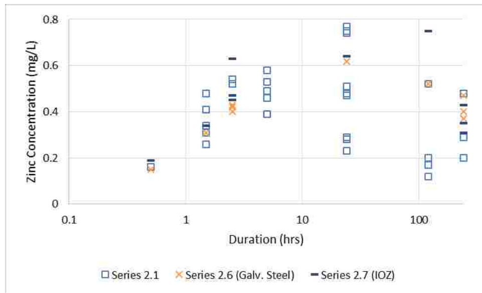
Figure 30. Series 2.6 and 2.7 zinc release
