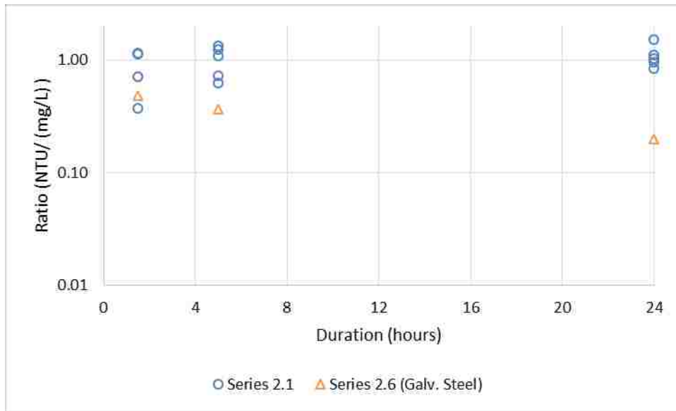
Figure 33. Theme 2 turbidity to concentration ratio
