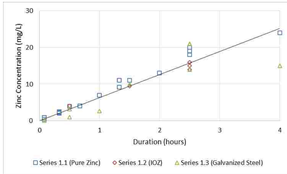
Figure 15. Prompt release at 85°C, first four hours
