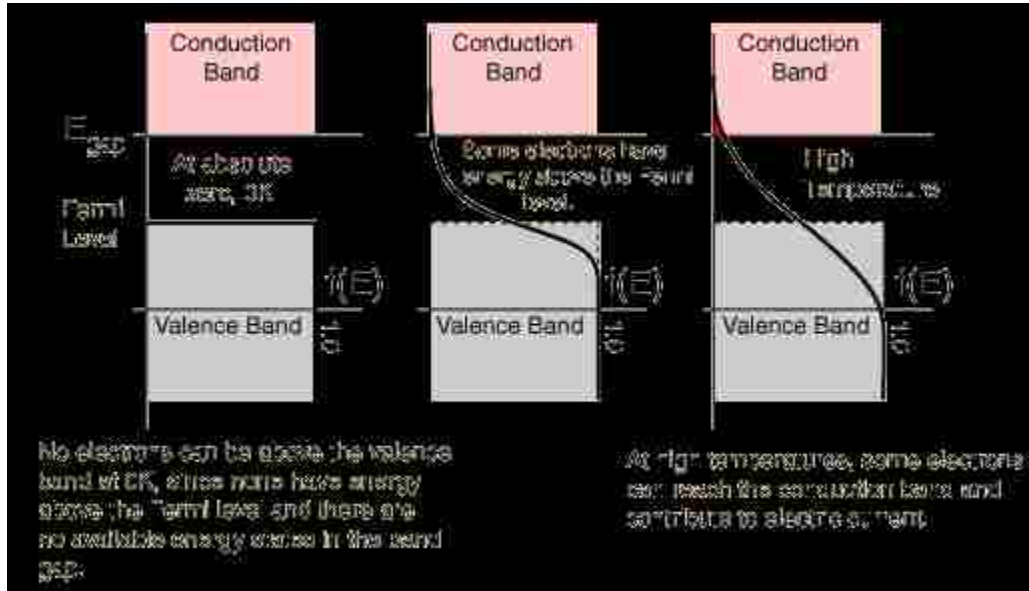
Figure 2. Fermi-Dirac distribution with increasing temperature [43]
