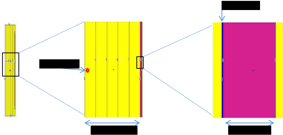
Figure 6. SSB detector geometry as modeled with MCNP5
