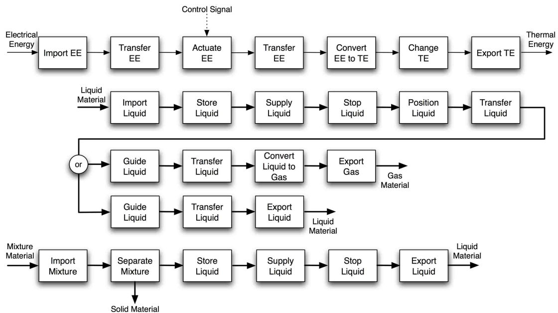
Figure 7. Tier 2 functional model of an ice tea maker
