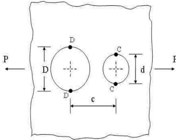
Figure 1.11. Infinite Plate with Two Circular Holes in Parallel Tension
