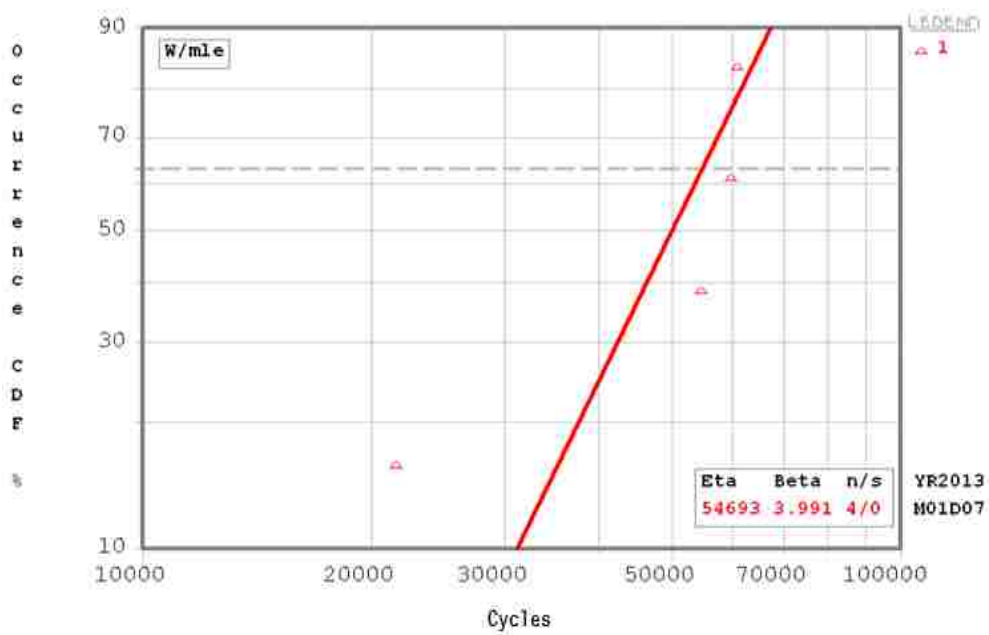
Figure 4.18. DW-OH-1000-1 thru 4 Characteristic Life Plot
