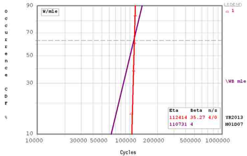
Figure 4.15. DW-OH-3079-1 thru 4 Characteristic Life Plot
