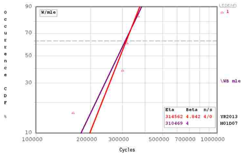
Figure 4.13. DW-RKt-1 thru 5 Characteristic Life Plot
