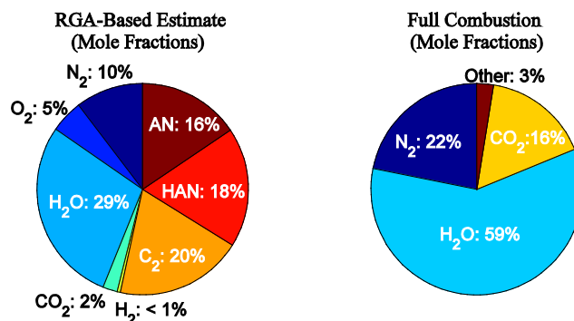
Figure 4.2: Plume exhaust gas species comparison.
