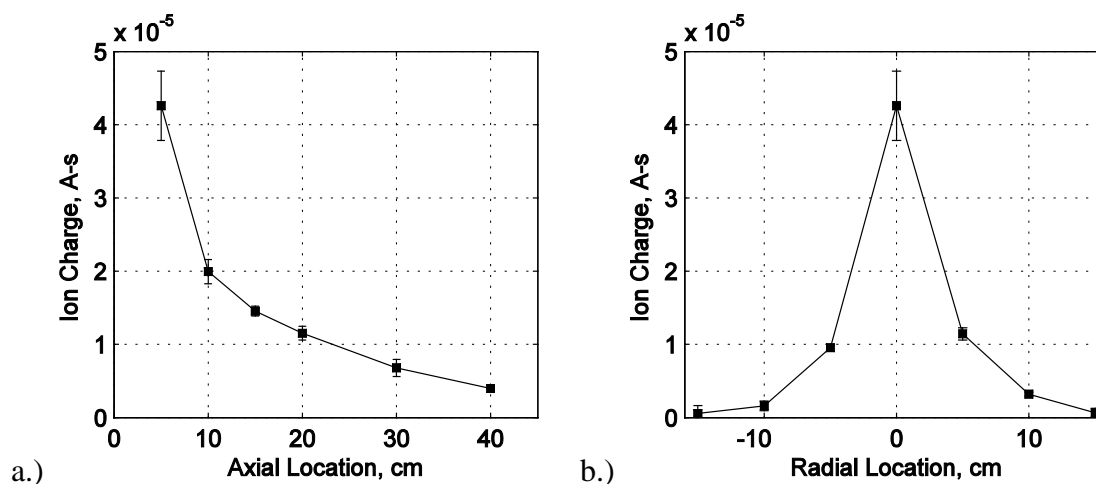
Figure 4.1: Integrated Faraday Probe results indicating total ion charge collected in Coulombs for the a.) centerline locations and b.) off-centerline locations.
