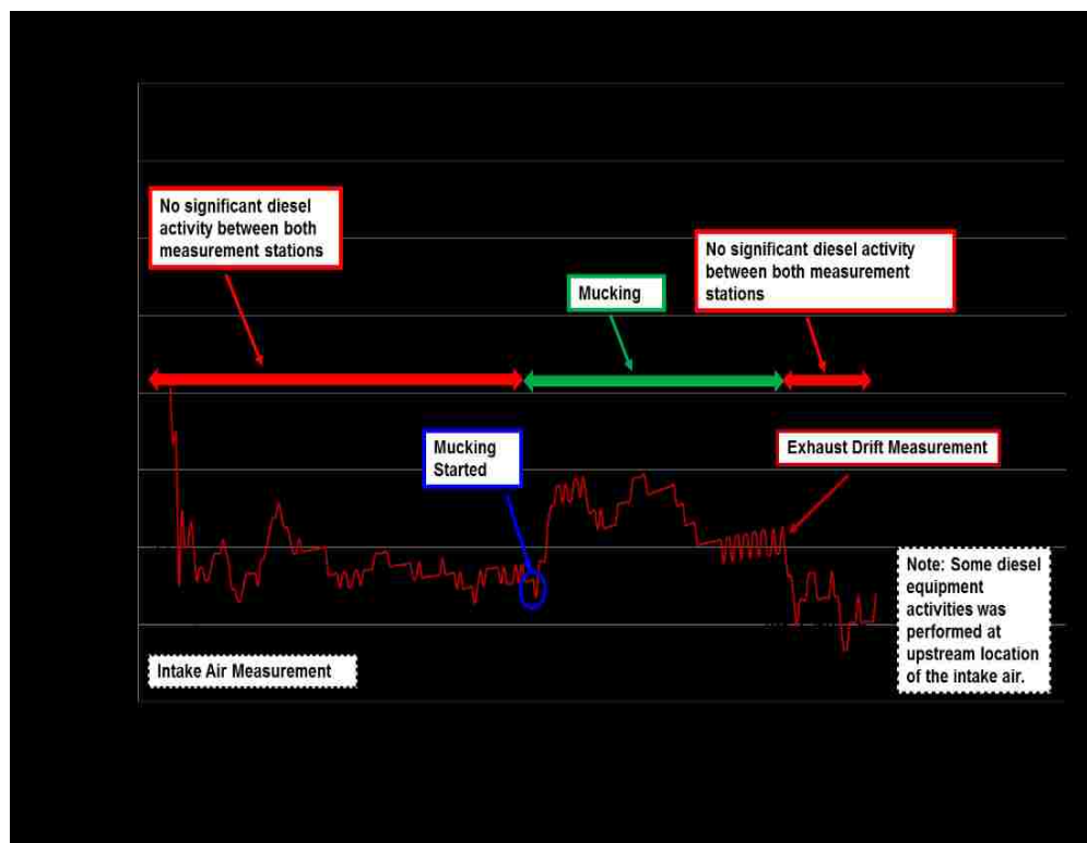
Figure 6.14 Inlet and exhaust air drifts EC during measurements A3
