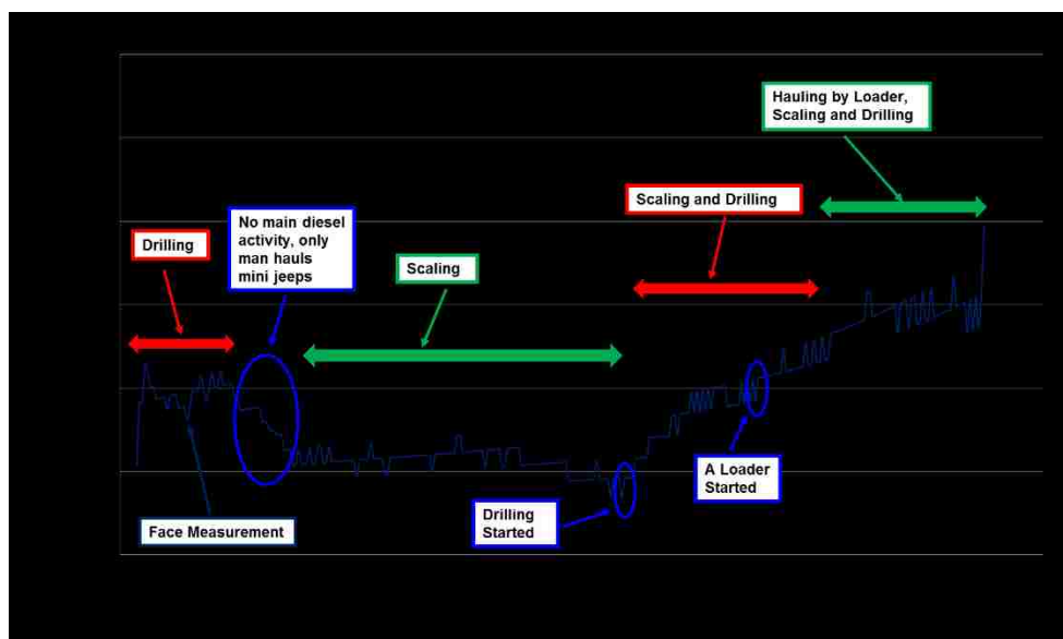
Figure 6.2 EC plot for work face measurement Z2
