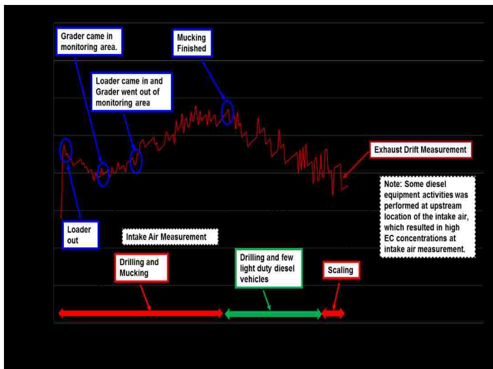
Figure 6.12 Inlet and exhaust air drifts EC during measurements A1
