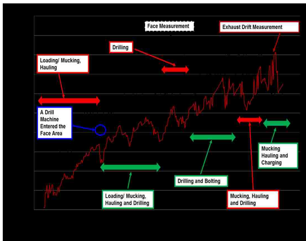
Figure 6.5 Work face and exhaust air drift EC during measurements B1
