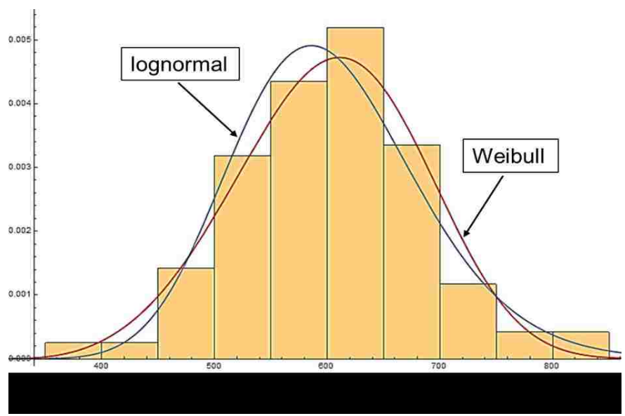
Figure 5.4 Frequency distribution plot of work face measurement D with lognormal and Weibull distribution fit
