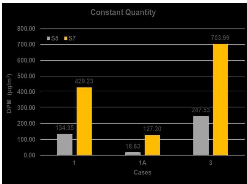
Figure 8.30 Average DPM for Case 1, Case 1A and Case 3 ( 19.5 \text{ m}^3/\text{s} )
