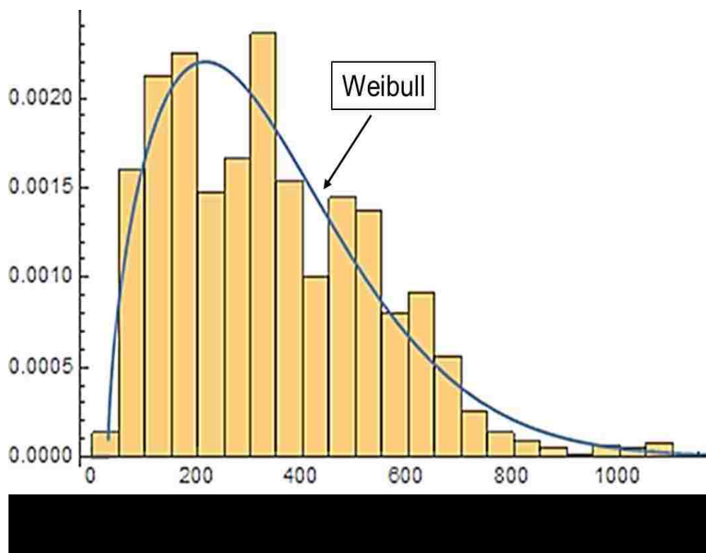
Figure 5.10 Frequency distribution of DPM concentrations during all work face measurements with Weibull distribution fit
