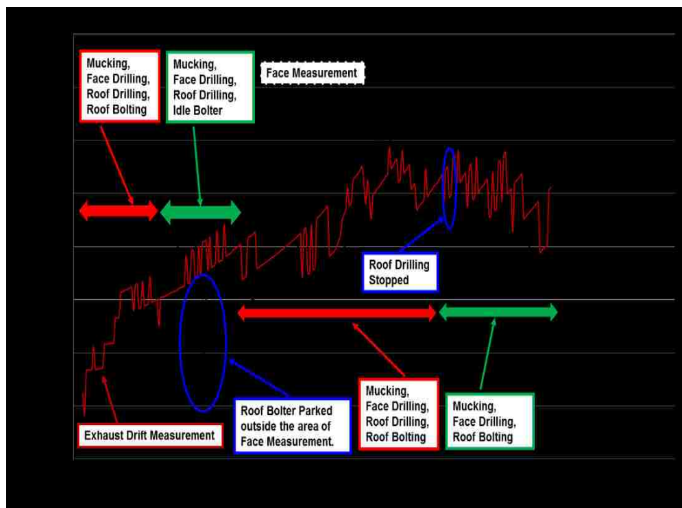
Figure 6.8 Work face and exhaust air drift EC during measurements B4
