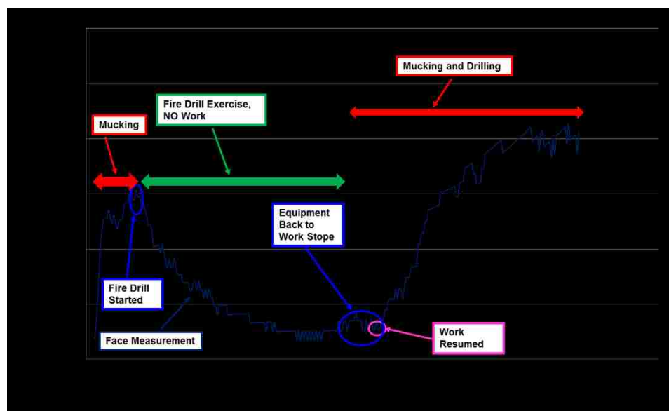
Figure 6.1 EC plot for work face measurement Z1
