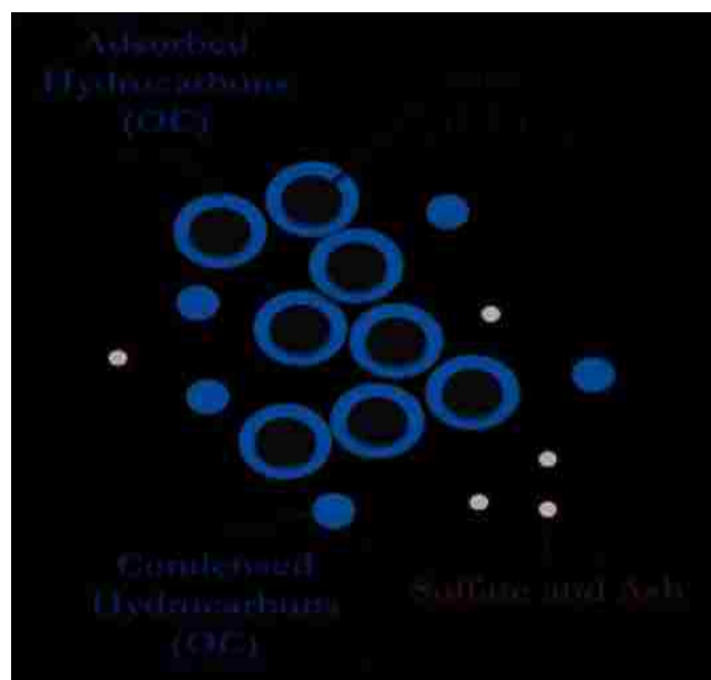
Figure 2.1 Diesel particulate matter composition
