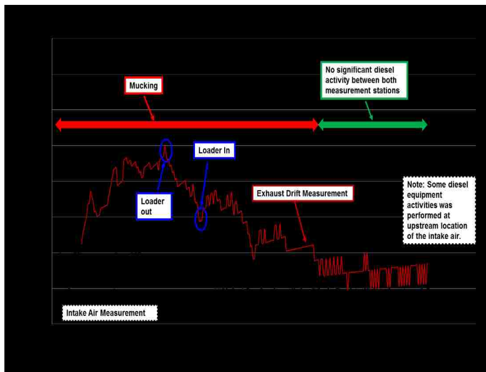
Figure 6.15 Inlet and exhaust air drifts EC during measurements A4
