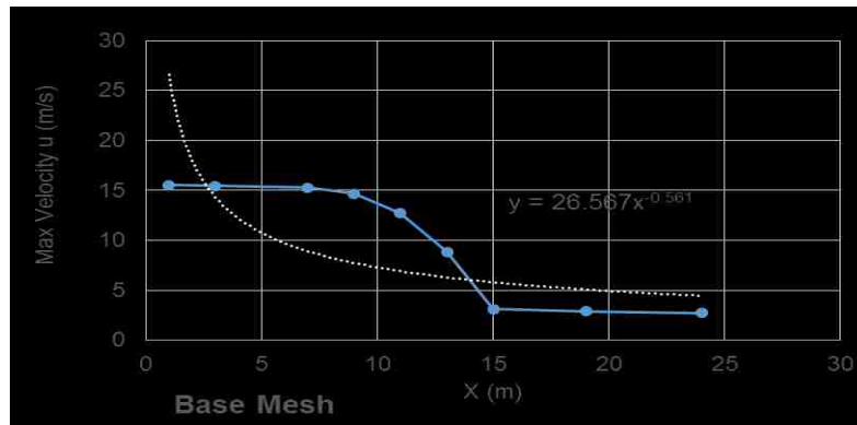
Figure 8.13 Maximum horizontal velocity vs distance in x direction for base mesh
