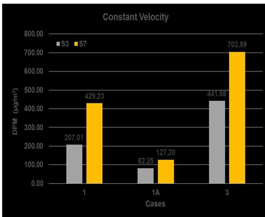
Figure 8.18 Average DPM for Case 1, Case 1A and Case 3 (10.0 m/s)
