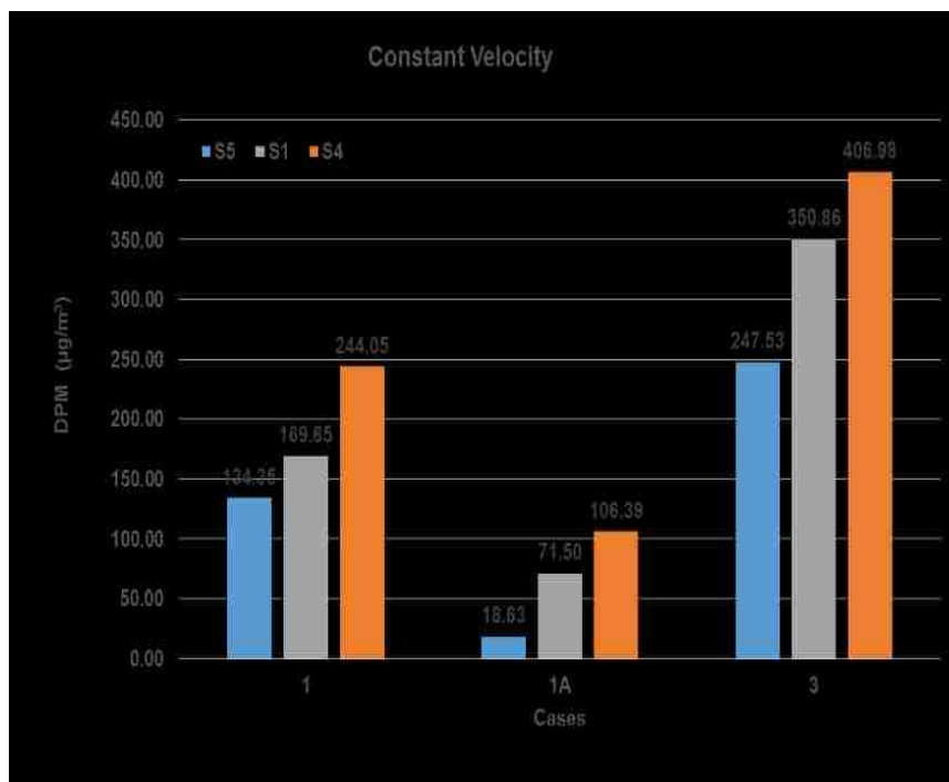
Figure 8.20 Average DPM for Case 1, Case 1A and Case 3 (15.5 m/s)
