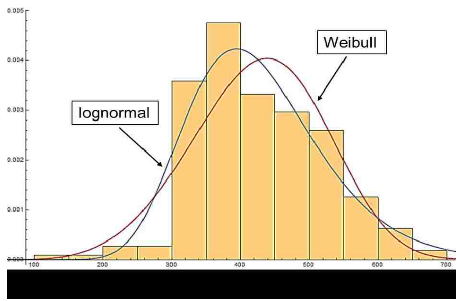
Figure 5.3 Frequency distribution plot of work face measurement C with lognormal and Weibull distribution fit
