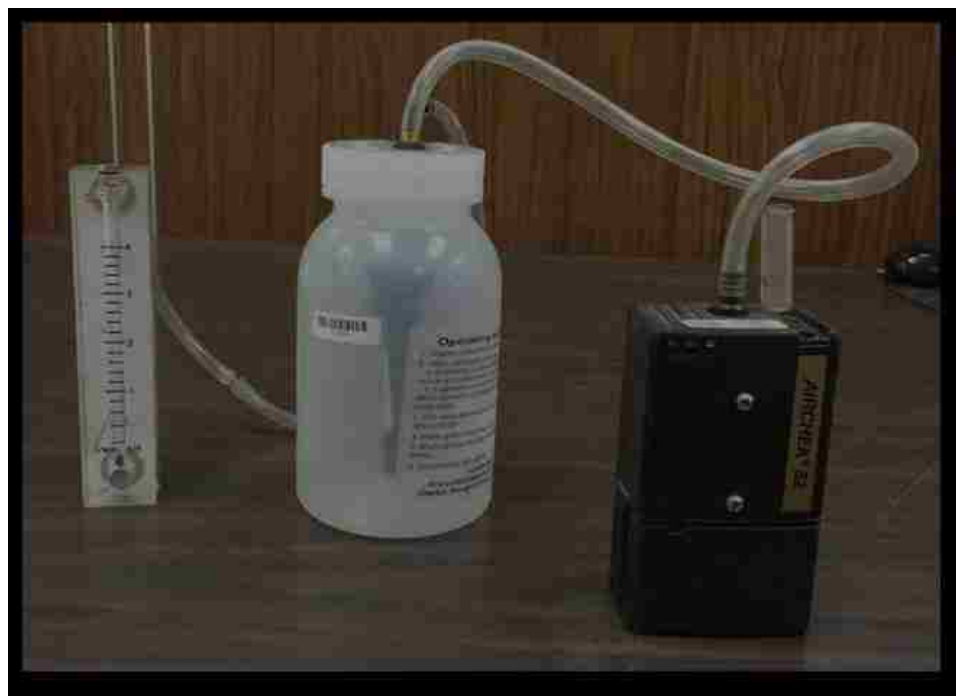
Figure 3.7 The NIOSH 5040 DPM sampling pump calibrations setup
