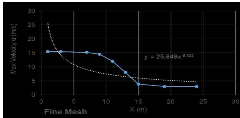
Figure 8.14 Maximum horizontal velocity vs distance in x direction for fine mesh
