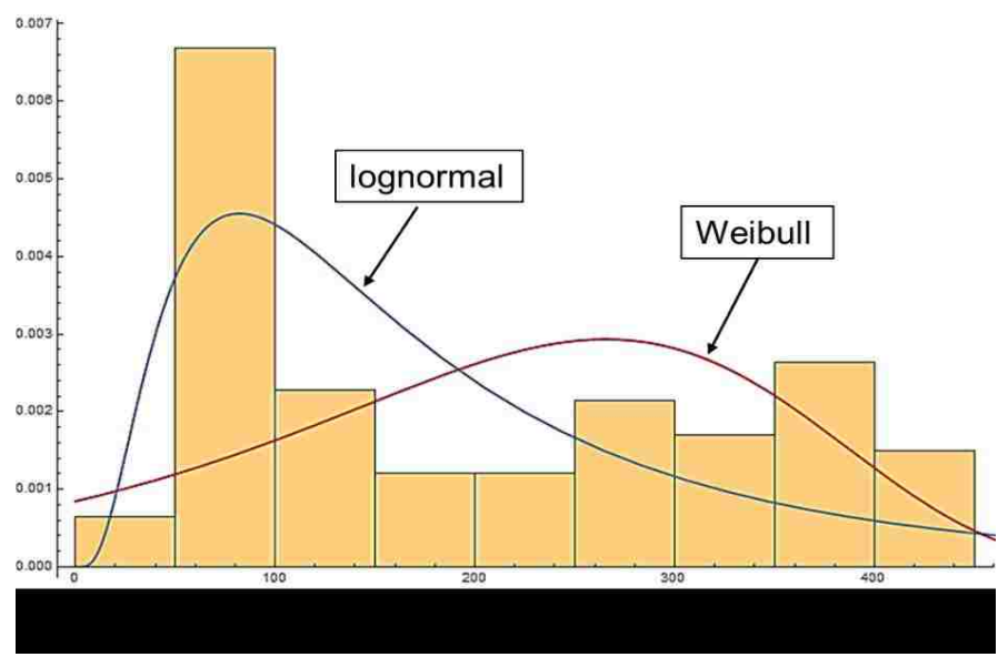
Figure 5.1 Frequency distribution plot of work face measurement A with lognormal and Weibull distribution fit
