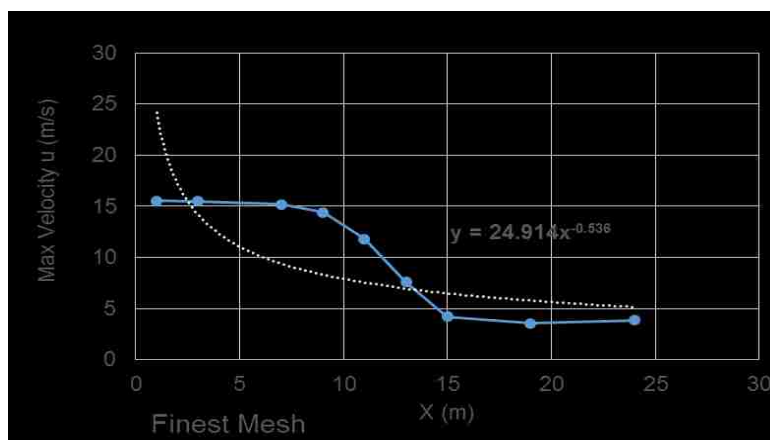
Figure 8.15 Maximum horizontal velocity vs distance in x direction for finest mesh
