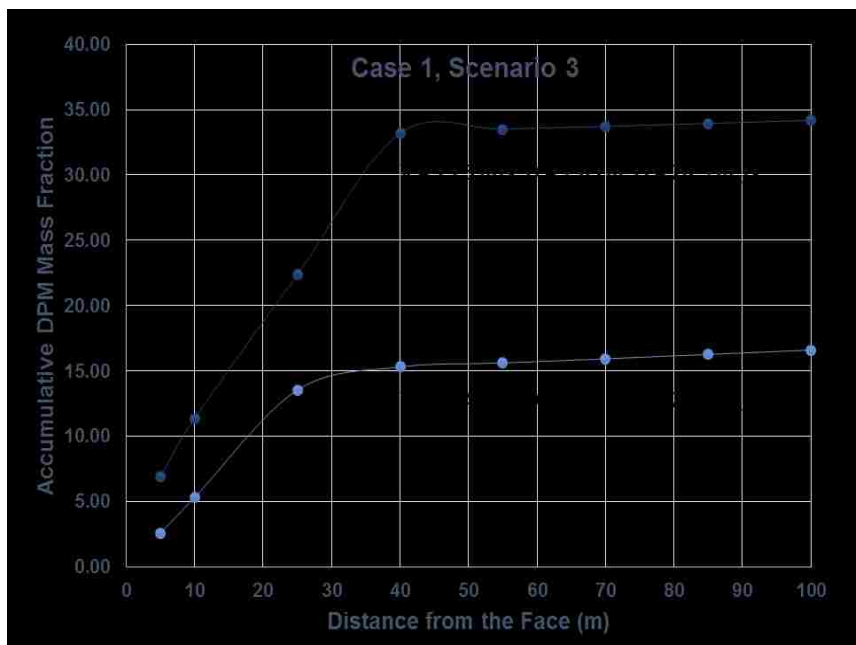
Figure 8.31 Accumulative DPM mass fraction versus face distance ( 28.9 \text{ m}^3/\text{s} )
