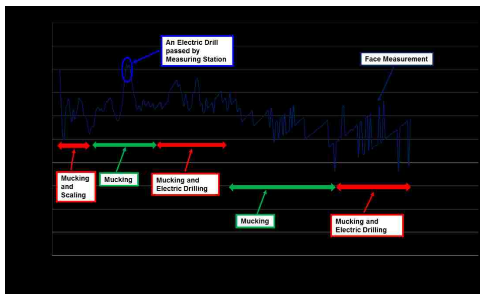
Figure 6.3 EC plot for work face measurement Z3
