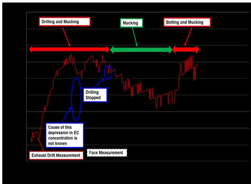
Figure 6.7 Work face and exhaust air drift EC during measurements B3
