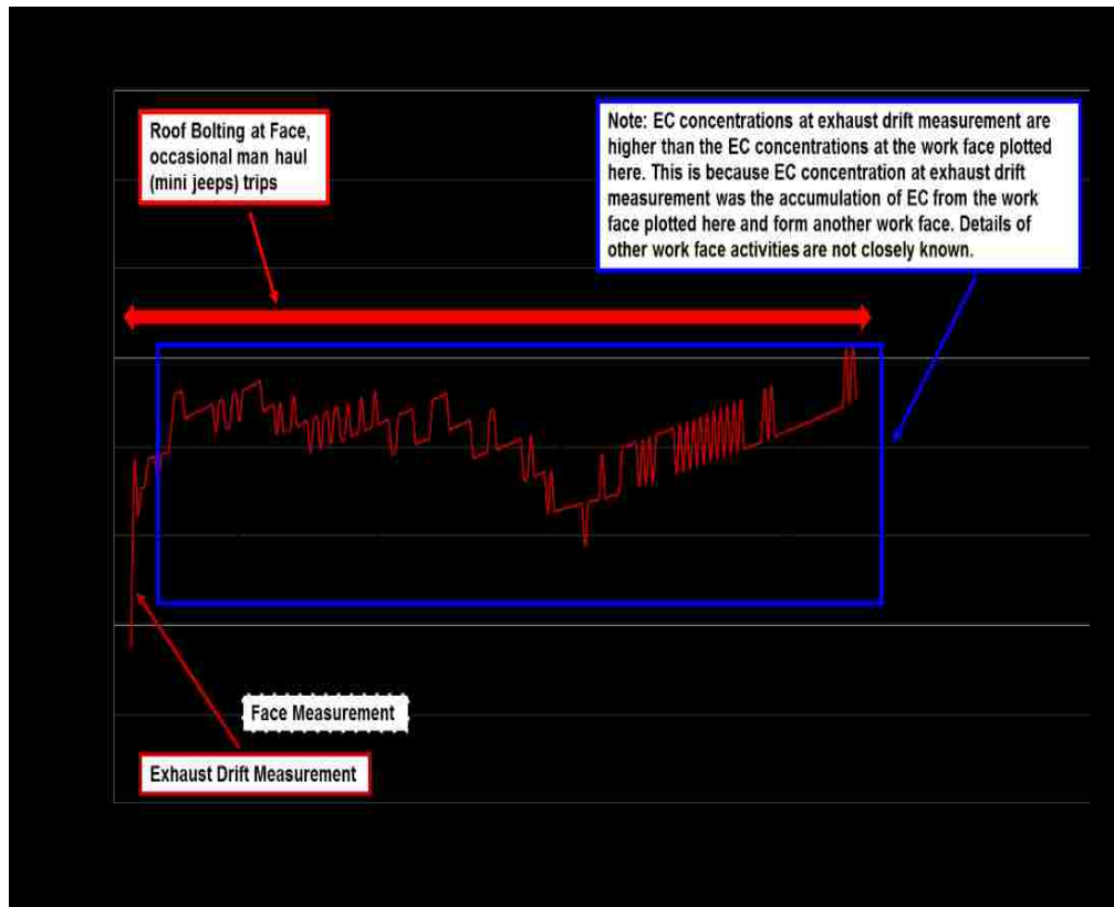
Figure 6.10 Work face and exhaust air drift EC during measurements B6
