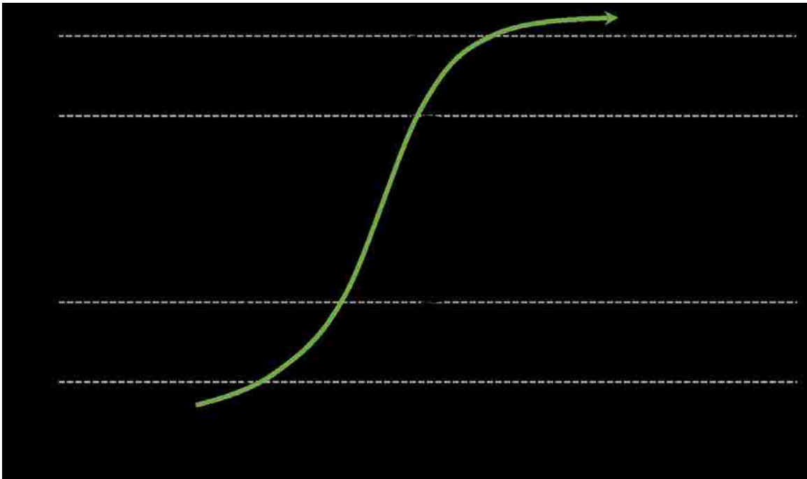
Figure 3.36. Standard growth curve with growth phases identified on the curve.
