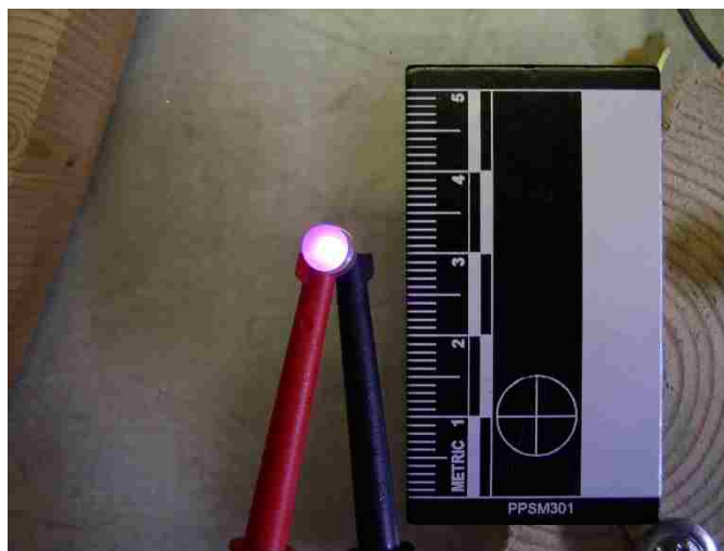
Figure 3.3. Experimental setup for taking spectroradiometric measurements with a 5 mm through-hole LED.
