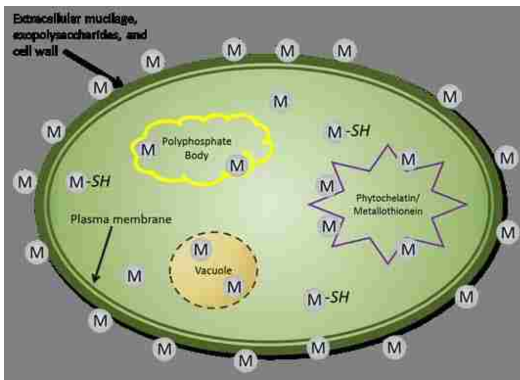
Figure 2.4. Diagram of the relative location and affinity of algal cell to metals in solution.
