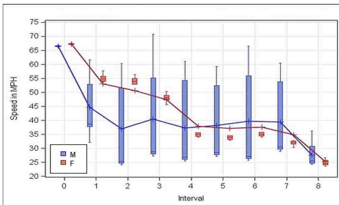
Figure 5.5 Box plot comparison for scenario-2
