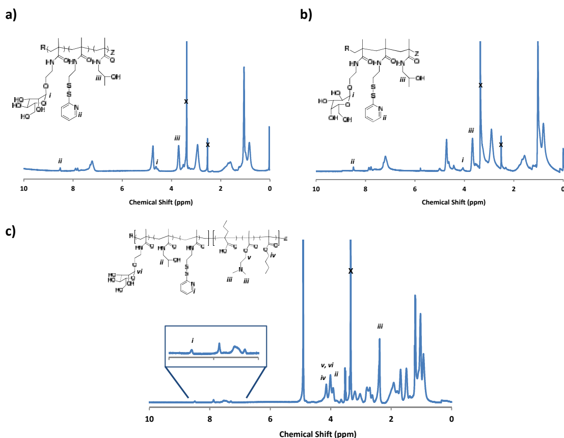
Figure 4.4 ^1\text{H-NMR} spectra in deuterated dimethyl sulfoxide (DMSO) of a) ManHPMA MacroCTA and b) GalHPMA MacroCTA. c) Representative ^1\text{H-NMR} spectrum in deuterated methanol ( \text{CD}_3\text{OD} ) of ManHPMAPDB diblock copolymer.
