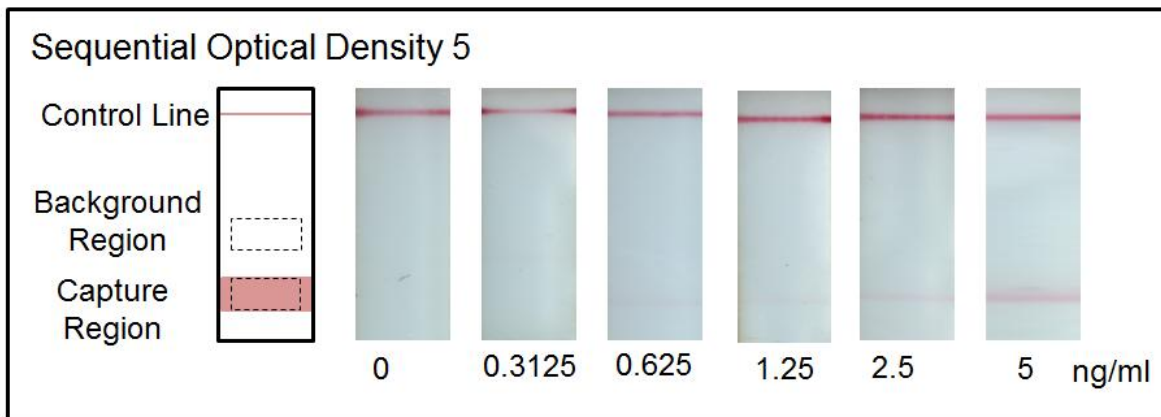
Figure 31. Sequential LOD assay results. Image series of the detection region for different concentrations of PfHRP2 analyte for sequential with OD 5 gold conjugate. At the far left is a schematic of the membrane with background, capture, and control line regions labeled. Dashed lines represent regions of analysis across a wide capture region.
