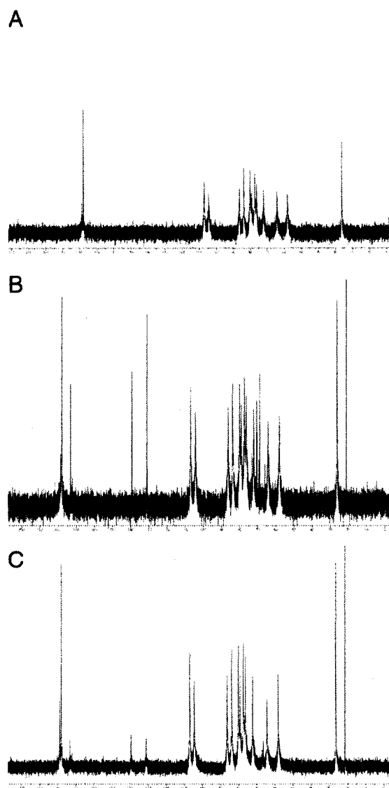
Figure 4.1: ^{13}\text{C} -NMR spectra of modified HAs. (A) Unmodified HA (220kDa). (B) HA(LMW)-GMA 1d, which resulted in hydrogels that were susceptible to hydrolysis. (C) HA(110)-GMA 5a, which resulted in hydrogels that were stable to hydrolysis.
