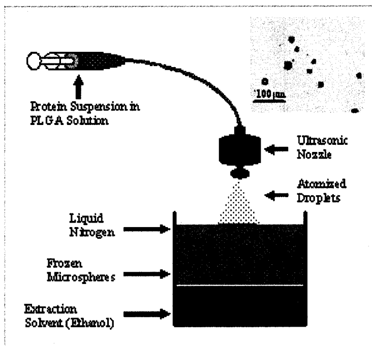
Figure 6.1: Microsphere fabrication using ProLease TM method. Protein is suspended in a PLGA solution, which is sprayed through an ultrasonic nozzle to form atomized droplets. The droplets are collected in a liquid nitrogen bath and allowed to freeze before entering a cold ethanol bath to extract the solvent. Inset shows brightfield micrograph of PLGA microspheres made using this method.
