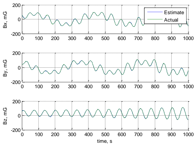
Figure 6.9. Magnetic Field Vector Estimation for 3,000 km Altitude
