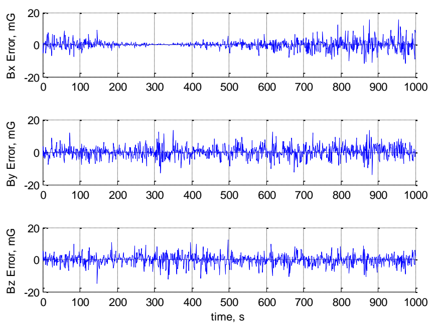
Figure 6.43. Magnetic Field Vector Estimation Error for Low Angular Velocity
