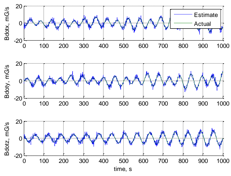
Figure 6.11. Magnetic Field Vector Derivative Estimation for 3,000 km Altitude
