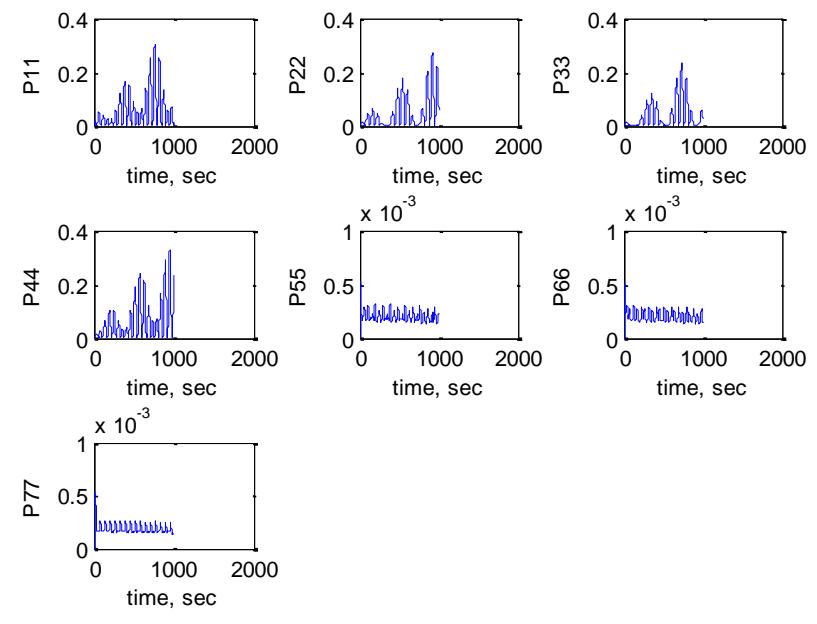
Figure 6.40. A Posteriori Error Covariance Estimation for Equatorial Orbit
