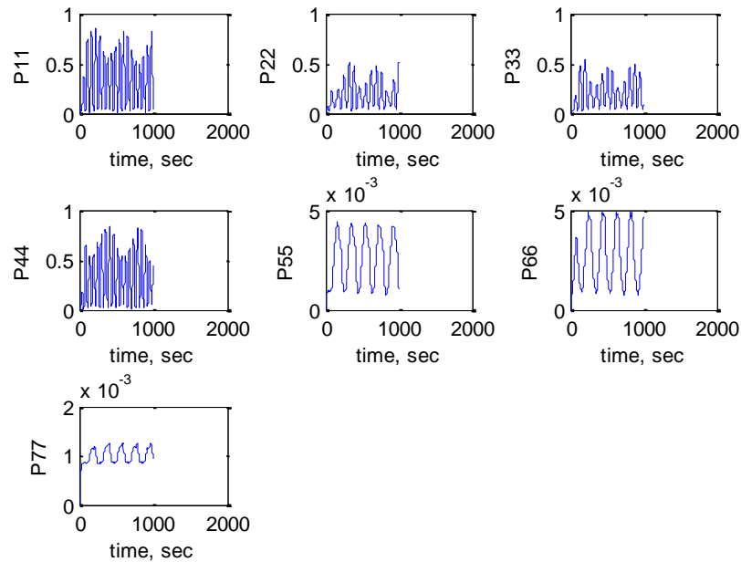
Figure 6.24. A Posteriori Error Covariance Estimation for 10,000 km Altitude
