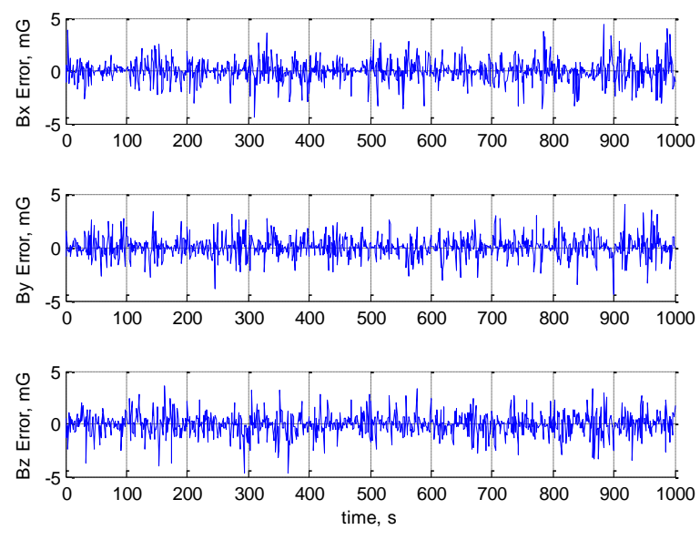
Figure 6.10. Magnetic Field Vector Estimation Error for 3,000 km Altitude
