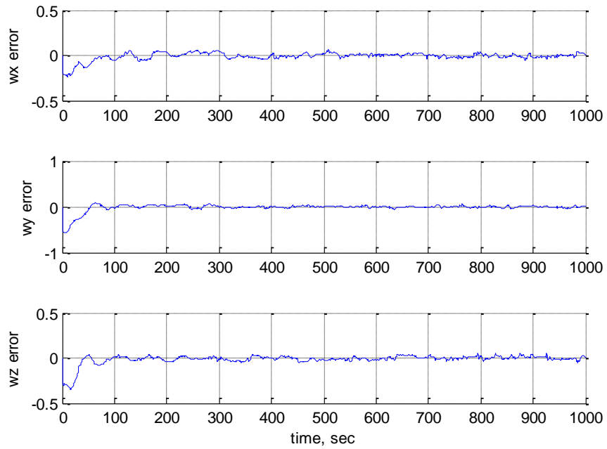
Figure 5.7. Angular Rate Estimation Error in Degrees/Second
