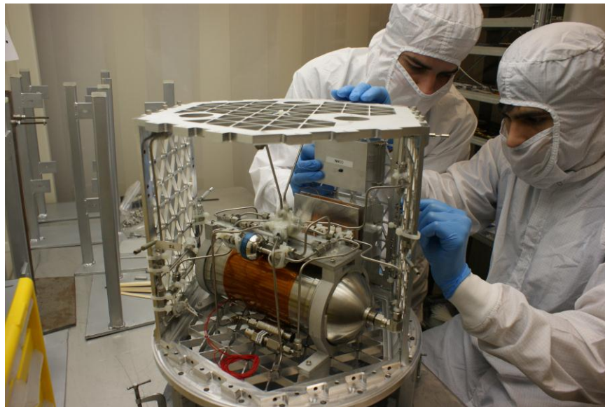
Figure 1.2. MR SAT Propulsion System Integration
