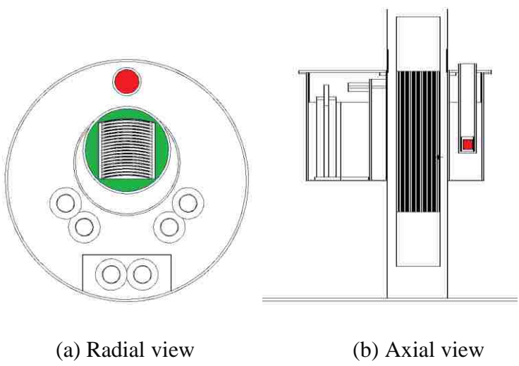
Figure 3-5: The combined MTR fuel assembly and AEFC experimental setup
