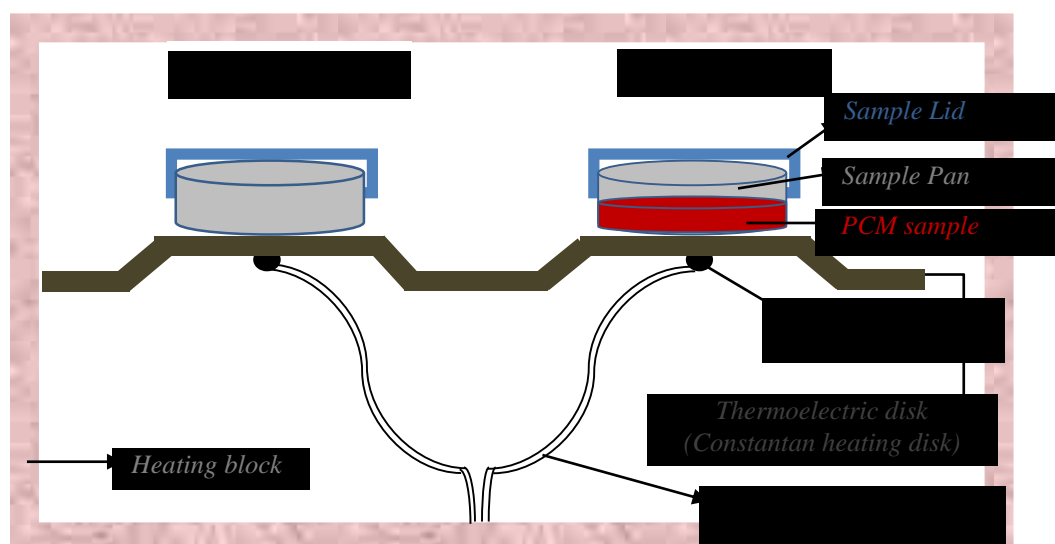
Figure 2.1. Schematic diagram of a typical DSC chamber
