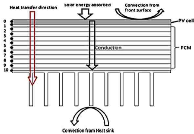
Figure 1.6. Sketch diagram of the experimental setup and PV panel configuration taken from [16].
