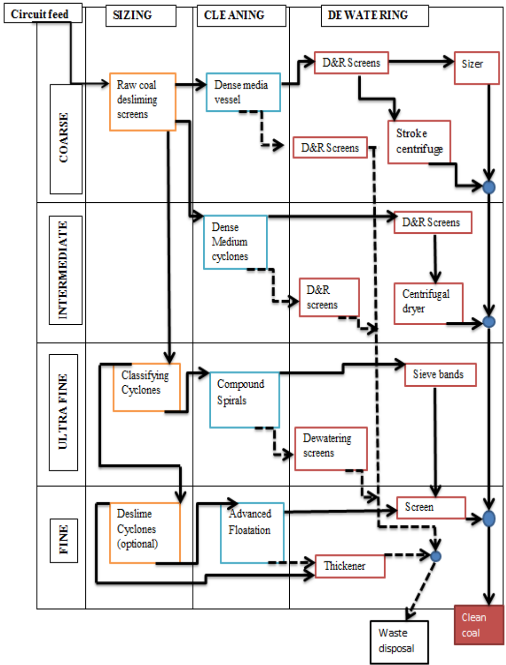
Figure 1.2. Typical coal cleaning circuitry
