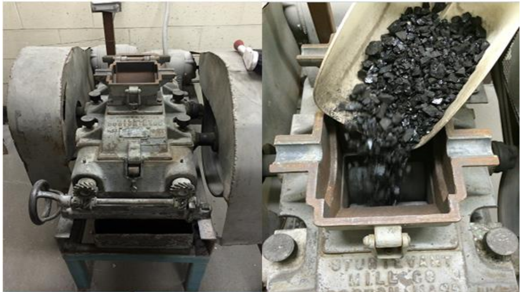
Figure 3.2.Laboratory Roll crusher
