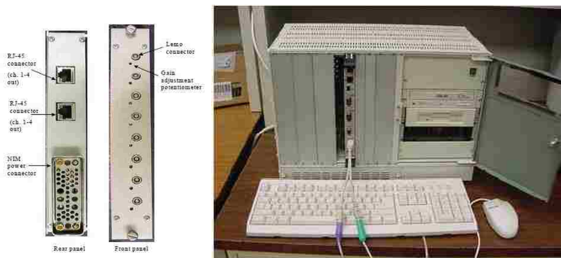
Figure 3.17: Shaping amplifier module (left) and the crate controller and single board computer (right)
