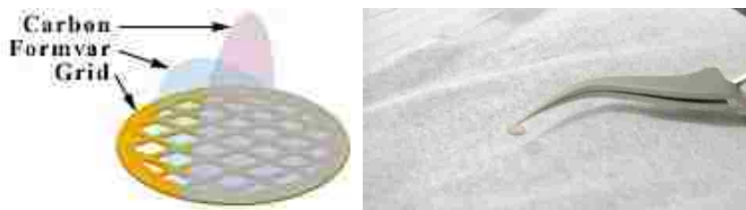
Figure 4.6. Schematic steps for sample preparation for STEM/TEM.
