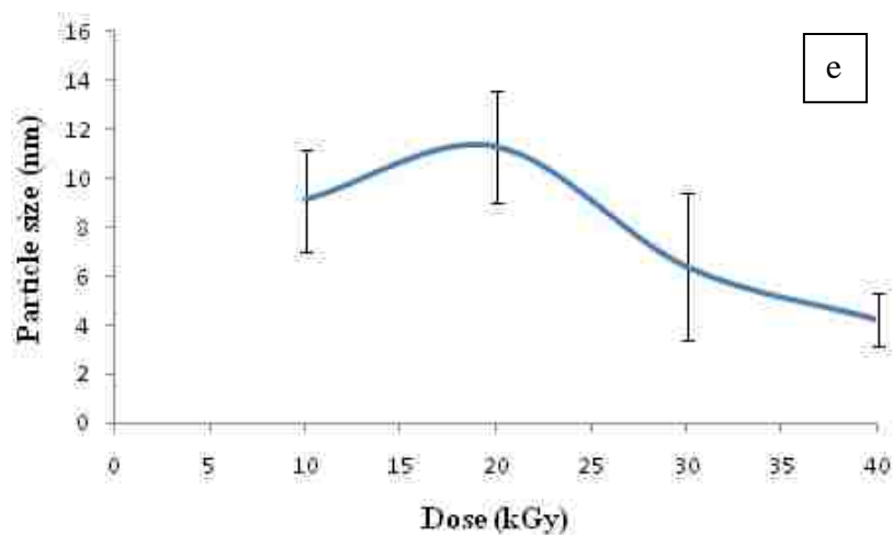
Figure 5.12. Particle size distribution of palladium nanoparticles at a) 10kGy b) 20kGy c) 30kGy, d) 40kGy and e) Plot of particle size vs. dose for \mu l (cont).
