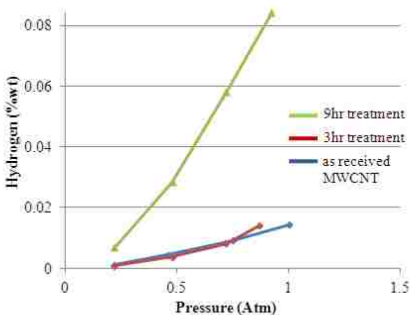
Figure A.1. Hydrogen storage capacity of MWCNTs treated with nitric acid for different periods of time. Measurements obtained up to 1 atm.
