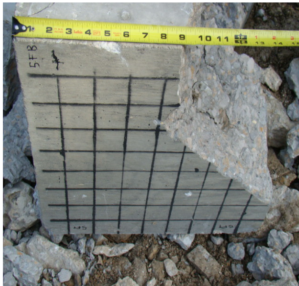
Figure 4.8: Block 5, front face after impact.
