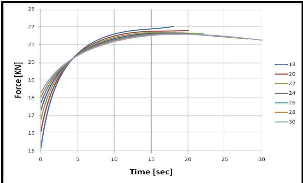
Figure 5.10 Simulation Experimentation Results: Piston Forces
