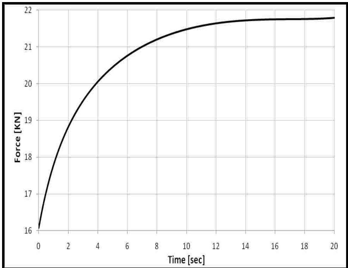
Figure 4.7 Force Output for 20 seconds Cycle Time Simulation
