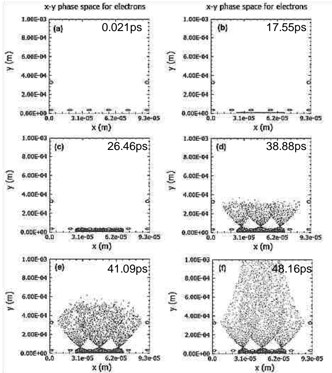
Figure 4.4. Trajectory of the beam of electron with focusing. Grid voltage: 45V, anode voltage: 30kV, focusing voltage: 4kV.
