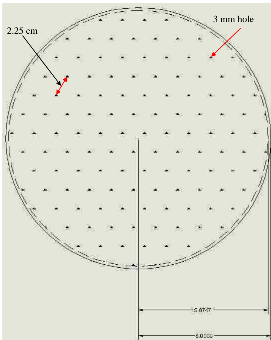
Figure 3.3. Schematic Diagram of the Air Perforated Distributor at the Exit of Upper Plenum (Figure 3.1), Units are in Inches
