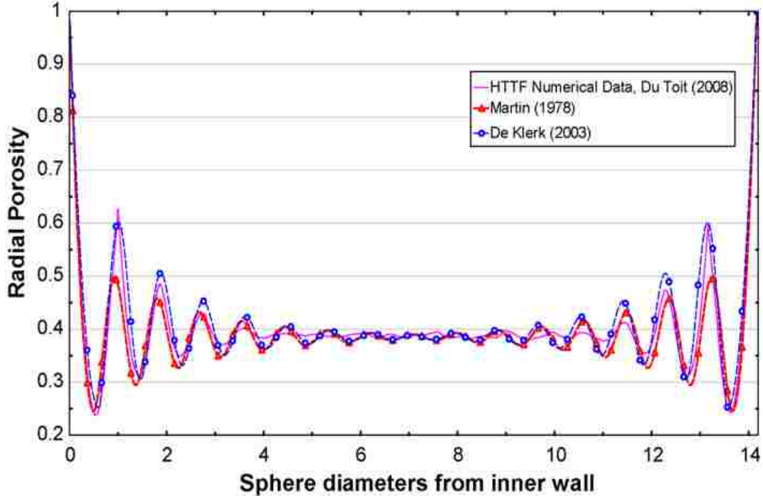
Figure 2.1. Comparison between Radial Oscillatory Porosity Correlations (van Antwerpen et al., 2010)
