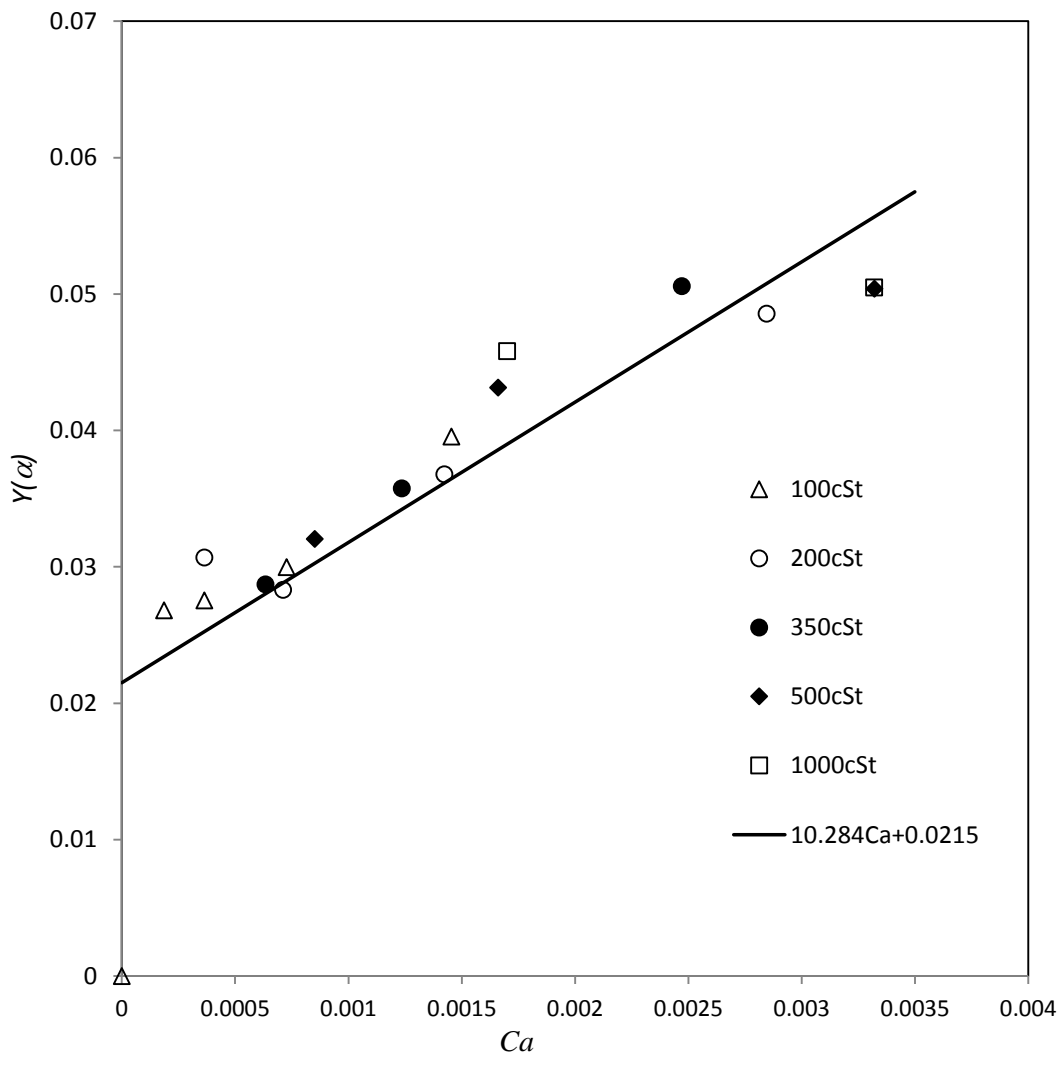
Figure 3.3. Receding contact angles versus capillary number with a best linear fit containing an intercept. Y(\alpha) has been calculated for Eq. (3) with reversed signs and using the data.
