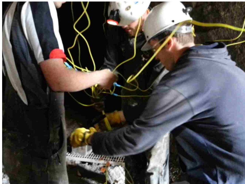
Figure A.4. Connecting individual detonating cords together
