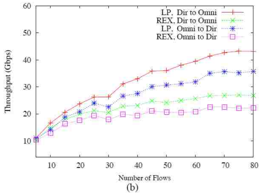
Fig. 4. Throughput
