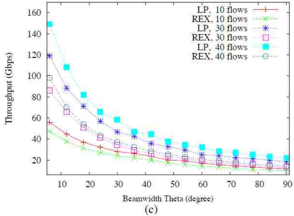
Fig. 3. Throughput (cont.)
