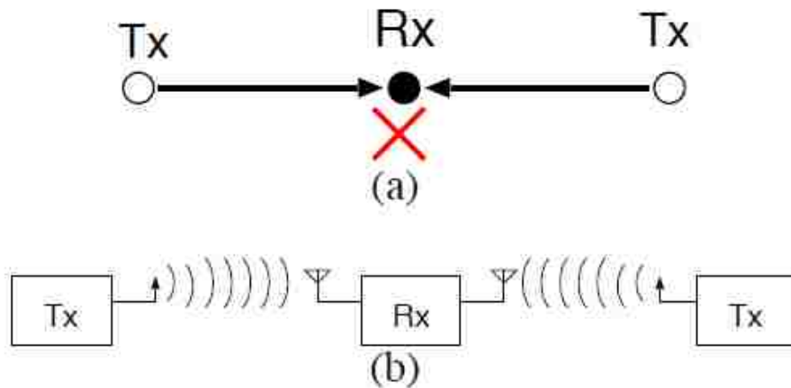
Fig. 1. Hidden Terminal Problem and MIMO Technology
