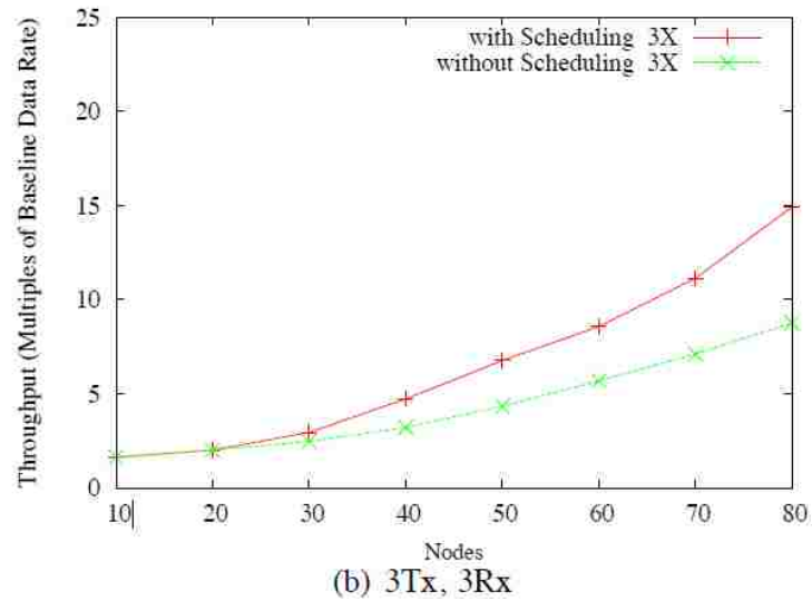
Fig. 3. R+S with Scheduling vs. R+S without Scheduling
