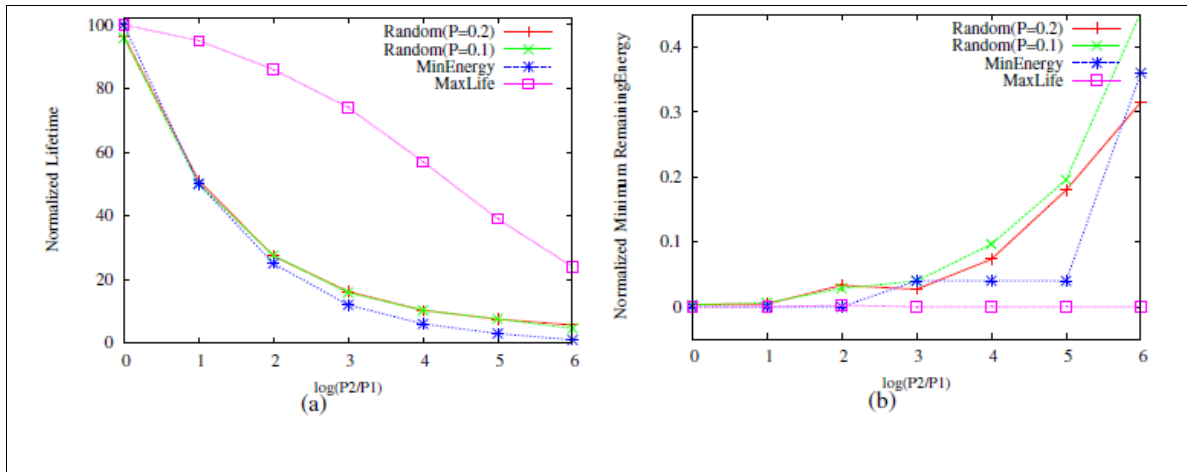
Fig.6.3 With initial energy reserve E = 1 , node-to-head P_1 = 0.01 , head-to-BS P_2 varies. (a) Functional lifetime (b) Remaining Energy after lifetime
