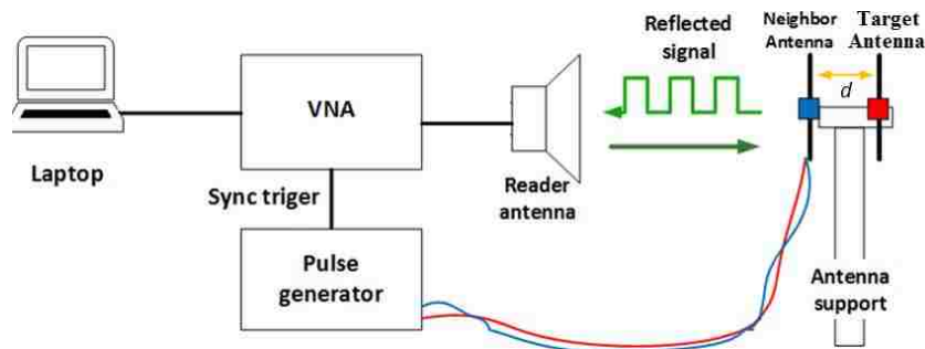
(b) Measurement setup
