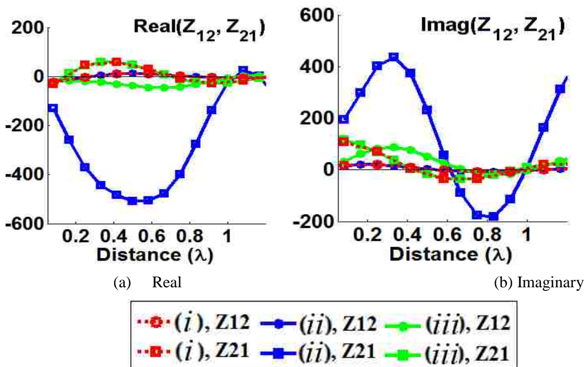
Figure 2.4. Simulated Real and Imaginary ( Z_{12} ) and ( Z_{21} ) for non-identical loads.
