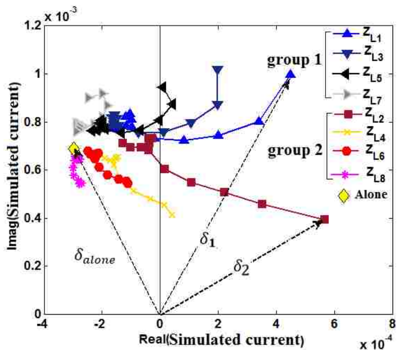
Figure 3.7. In front neighbor scenario loads in group 1 and 2 produce respectively constructive and destructive interference to the target antenna.
