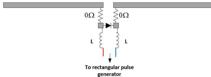
(a) Prepared half-wave dipole for measurements
