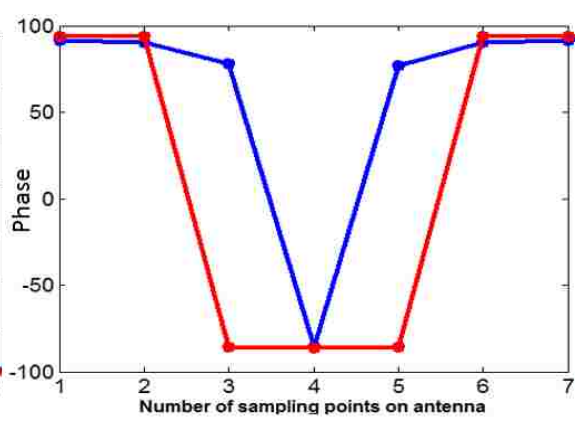
(c) Phase of current distribution
