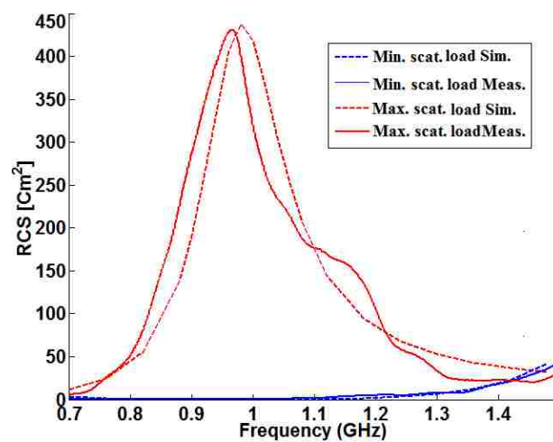
Figure 4.2. Simulated and measured RCS from min/max scattering antennas.
