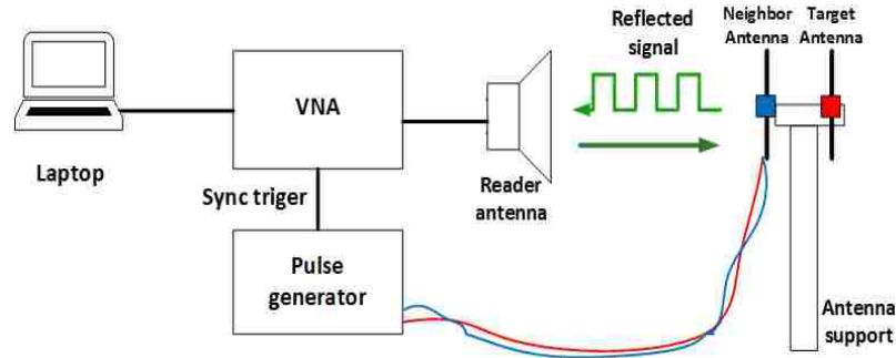
Figure 4.2. Measurement setup [15].
