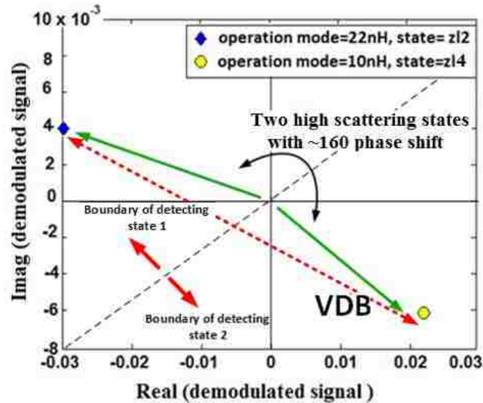
Figure 3.3. Two high scattering states with approximately \sim\Delta\varphi = 160^\circ .
