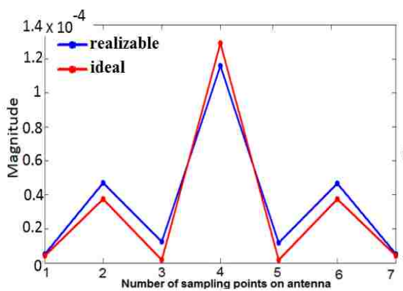
(b) Magnitude of current distribution
