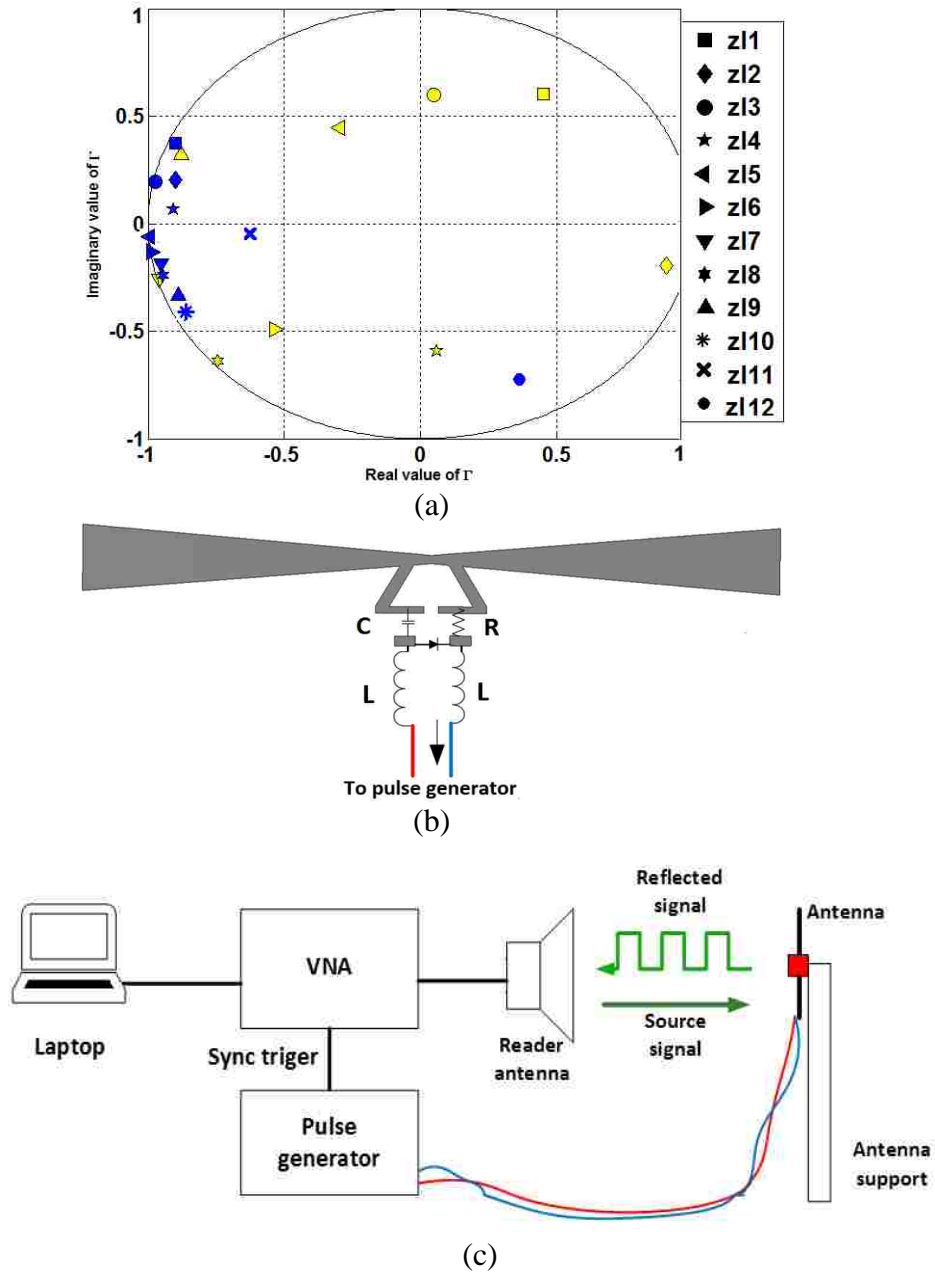
Figure 2.4. (a) Load impedances from each antenna's \Gamma plane are selected and are shown on a common \Gamma plane. The impedance of the diode in its forward bias ( 1\Omega + 0.7nH ) is also added to the total load at the input port of the antennas. (b) Prepared T-match antenna for measurements (c) Measurement set up.
