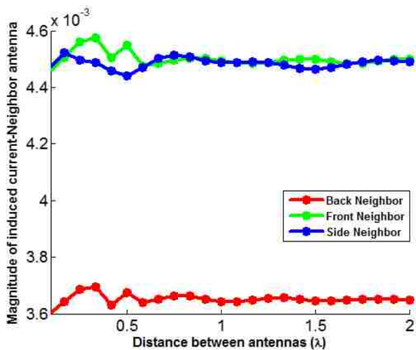
(b) Magnitude of current at the neighbor antenna
