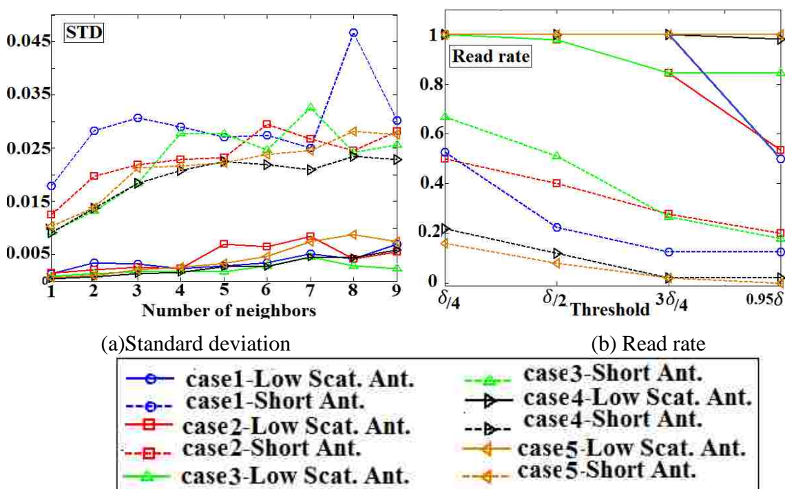
Figure 4.7. (a) Standard deviation of demodulated signal from the alone state at target antenna (b) read rates.
