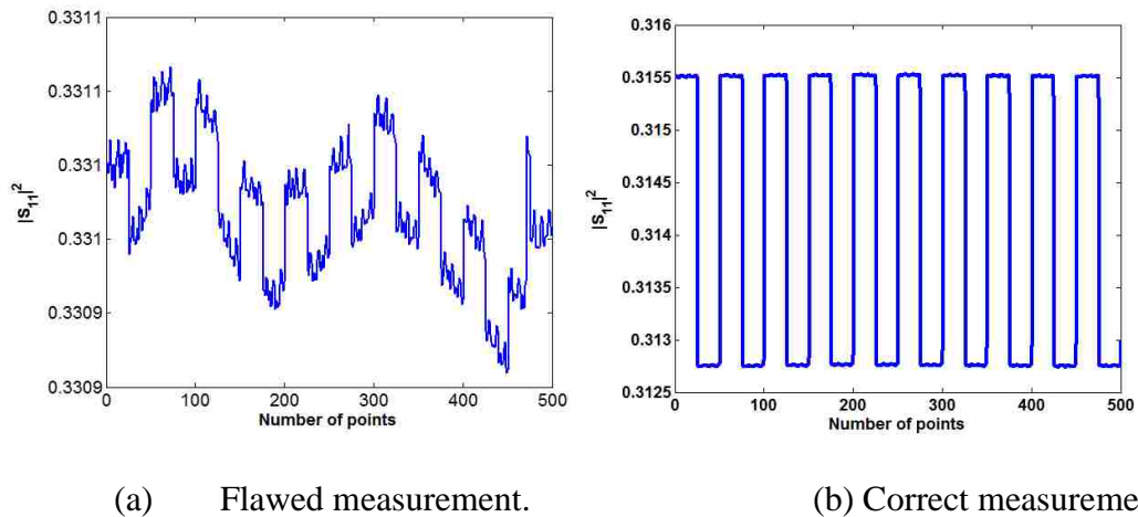
Figure 4.3. The measured S_{11} at VNA.
