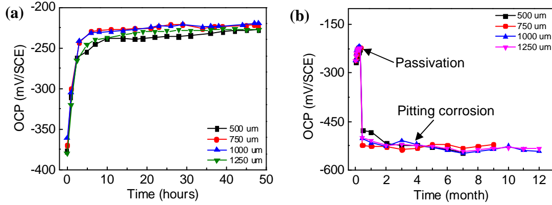
Figure 5.6. OCP in saturated \text{Ca(OH)}_2 solution: (a) without NaCl and (b) with NaCl.
