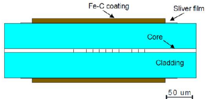
Figure 4.1. Schematic illustration of the structure of a Fe-C coated LPFG.
