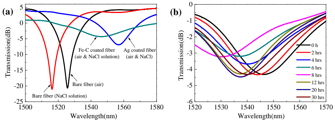
Figure 2.3. Transmission spectra of an LPFG sensor (a) coated and uncoated when tested in air and 3.5wt. %NaCl solution immediately, (b) coated with Ag (800 nm) and Fe-C (8 \mu\text{m} ) layers when tested in 3.5 wt. % NaCl solution over time.
