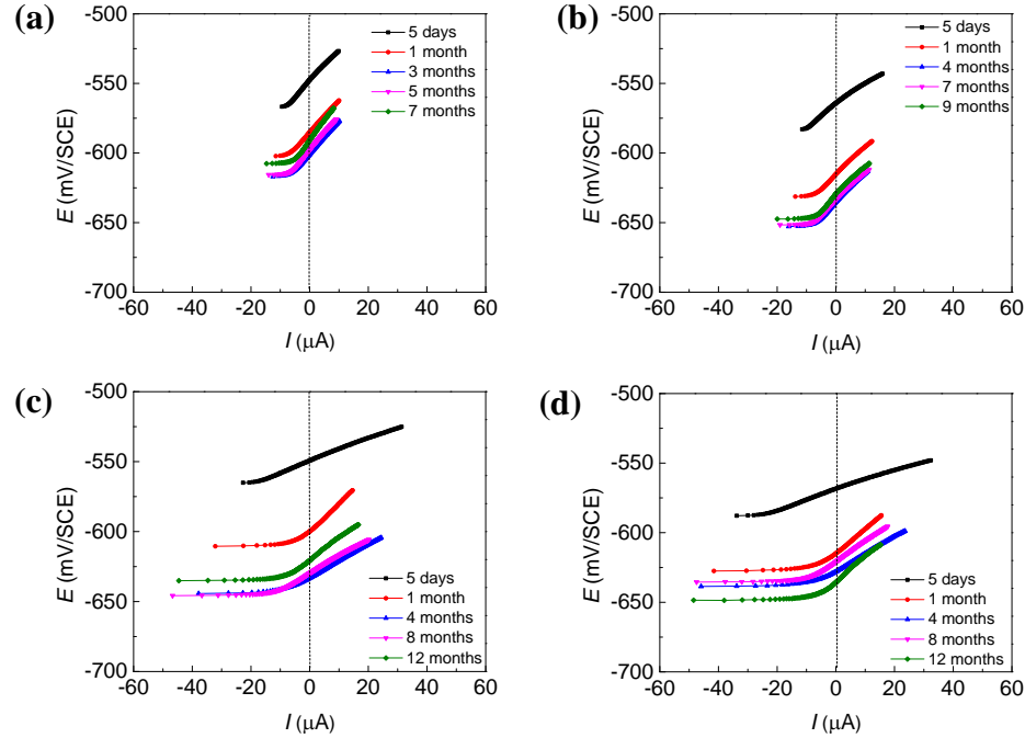
Figure 5.7. LPR of four steel tubes with wall thickness of: (a) 500 \mu m, (b) 750 \mu m, (c) 1000 \mu m, and (d) 1250 \mu m.
