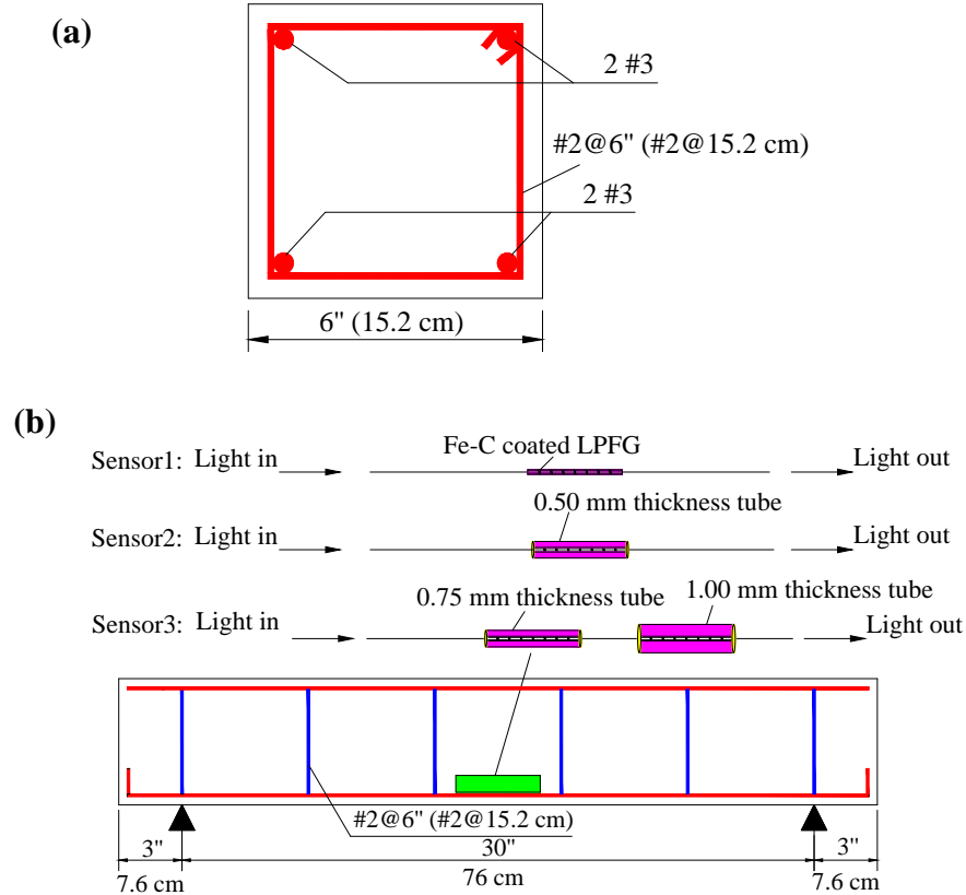
Figure 7.1. RC beam specimen and instrumentation:(a) cross section (b) reinforcement detail and instrumentation plan.
