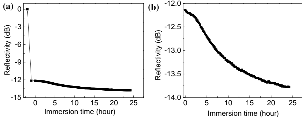
Figure 5.3. Change of reflectivity over time: (a) from air to 3.5 wt. % NaCl solution and (b) in the solution only.
