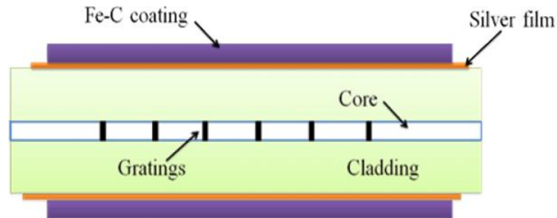
Figure 2.1. Schematic view of a Fe-C coated LPFG sensor.
