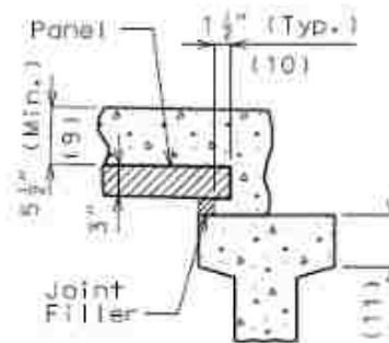
Figure 2.4 Typical panel-concrete girder joint detailing (MoDOT, 2016) Conversion: 1 in. = 25.4 mm
