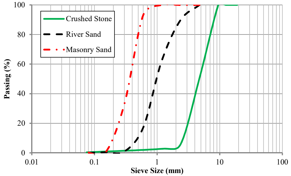
Figure 4.2. Gradation of the aggregates used
