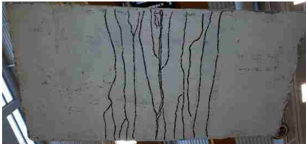
Figure 6.22. Crack pattern formation at the tension face of panel FUW2
