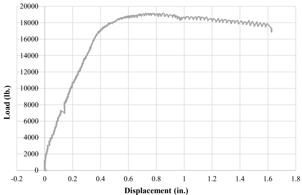
Figure 6.12. Load versus displacement for panel FUC3 Conversion: 1 in. = 25.4mm; 1 lb. = 4.45 N
