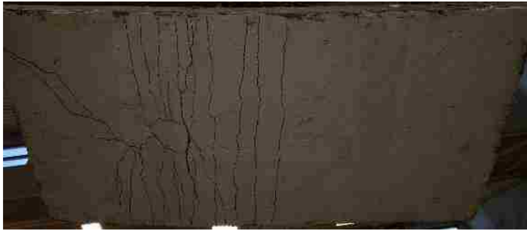
Figure 6.50. Crack pattern formation at the tension face of panel SUC2
