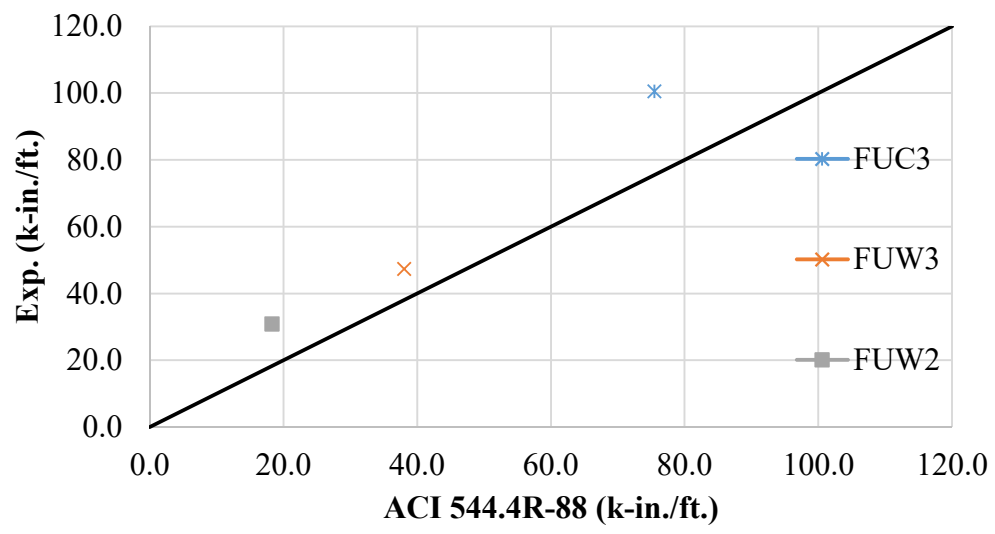
Figure 6.34. Empirical versus ACI 544.4R-88 moment values for flexure panels Conversion: 1 k-in./ft. = 0.371 kN.m/m
