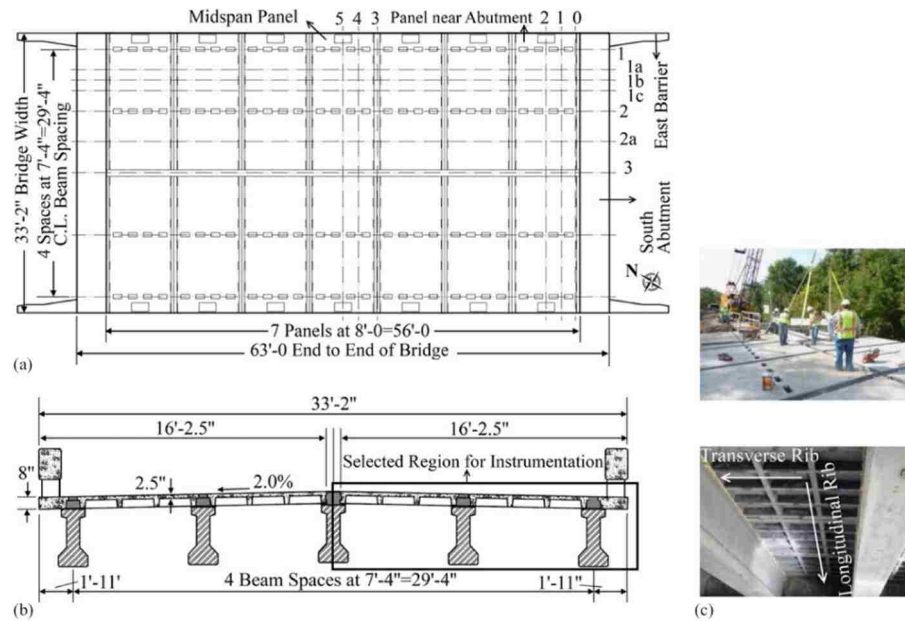
Figure 2.8. Dahlongea Road Bridge (a) plan view; (b) cross section; (c) during construction (Aaleti et al., 2015)
