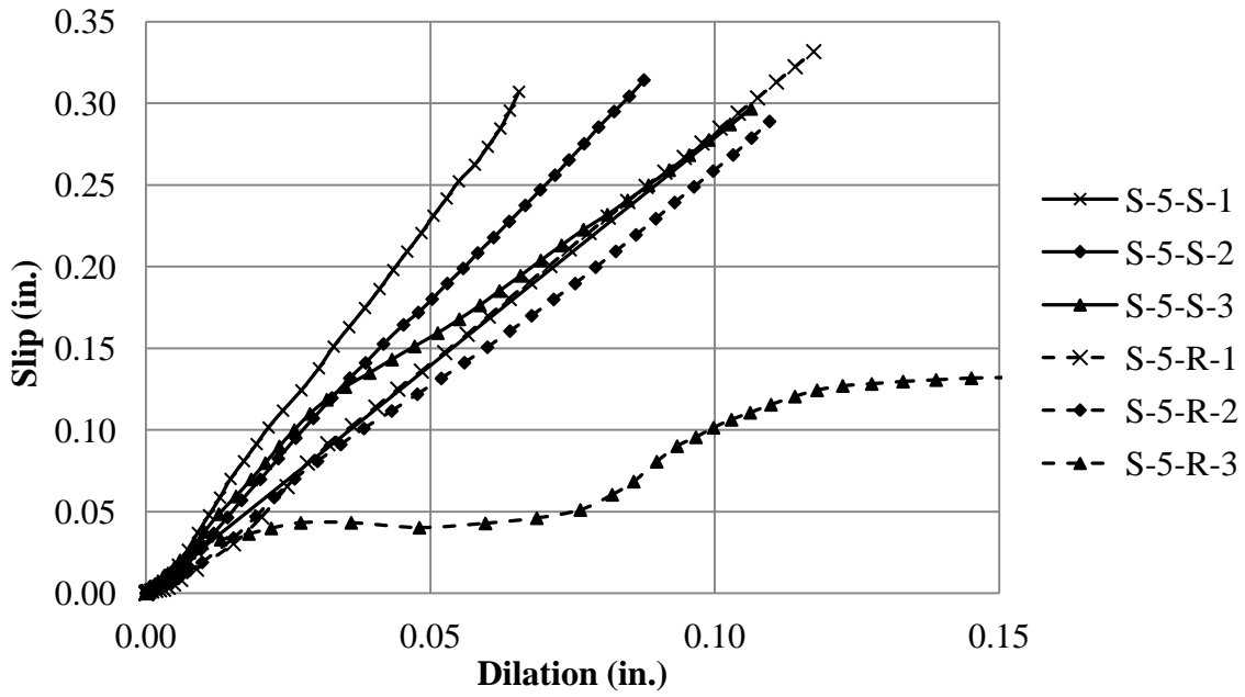
Figure 3.29. Slip vs. dilatation for 5000 psi sand-lightweight concrete specimens
