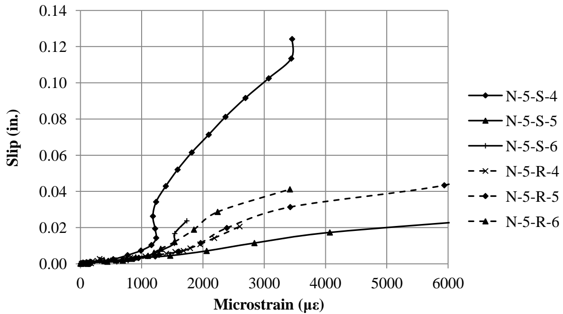
Figure 3.21. Slip vs. interface steel strain for 5000 psi normalweight concrete specimens
