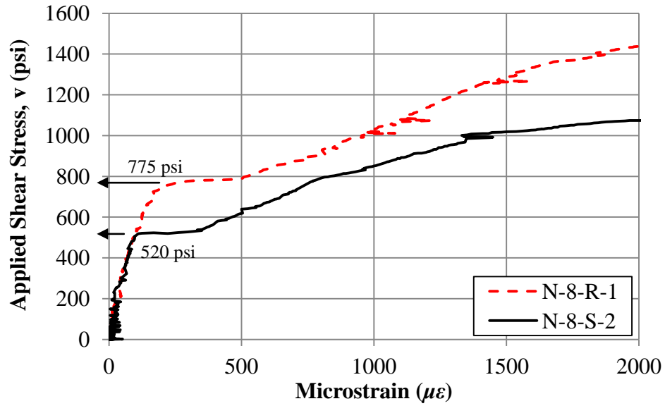
Figure 4.2. Typical shear stress-interface reinforcement strain plots for the determination of interface cracking stress (Specimens N-8-S-2 and N-8-R-1 shown)
