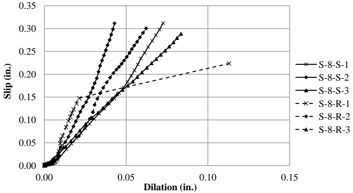
Figure 3.35. Slip vs. dilation for 8000 psi sand-lightweight concrete specimens
