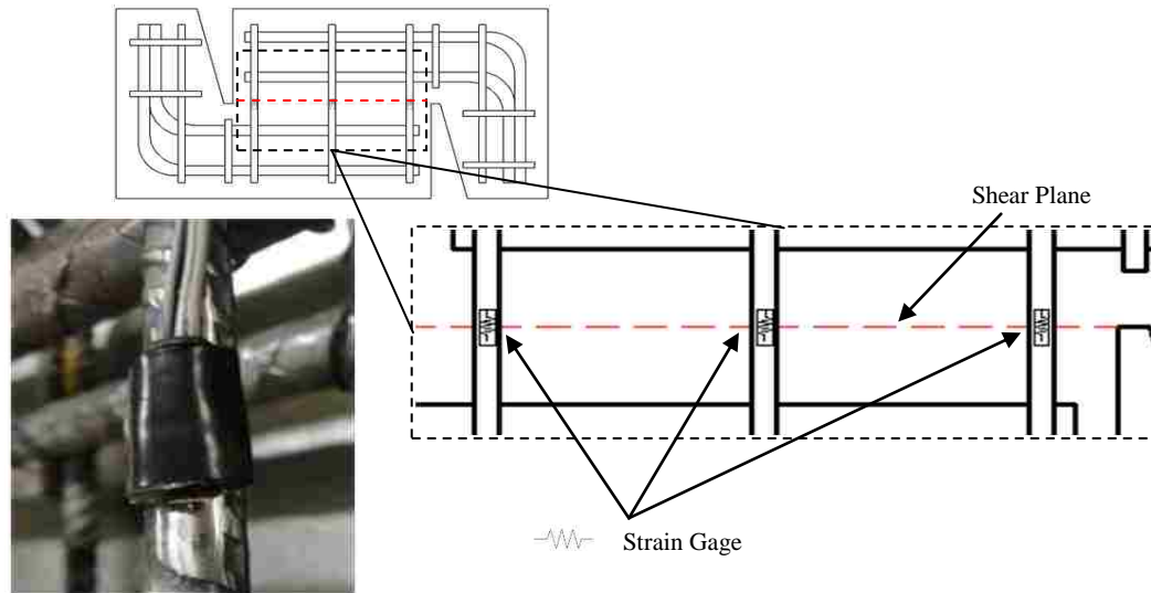
Figure 3.16. Strain gage protection and locations
