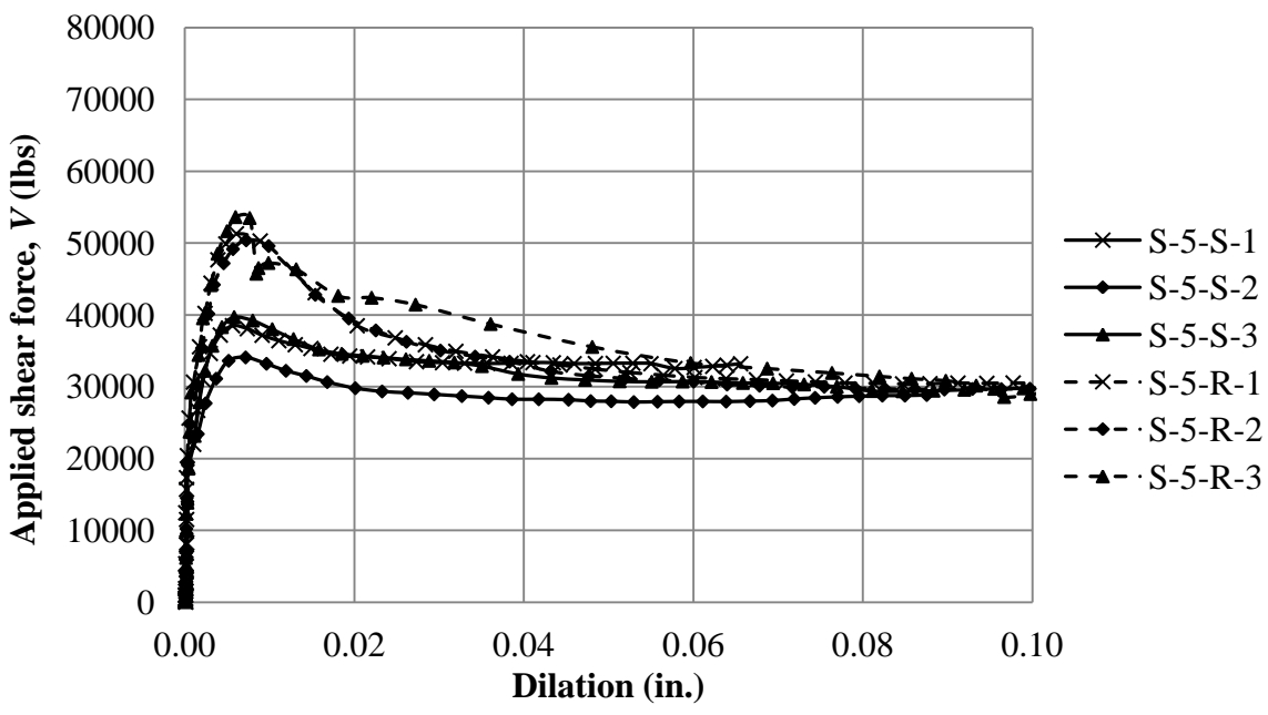
Figure 3.28. Applied shear force vs. interface dilatation for 5000 psi sand-lightweight concrete specimens
