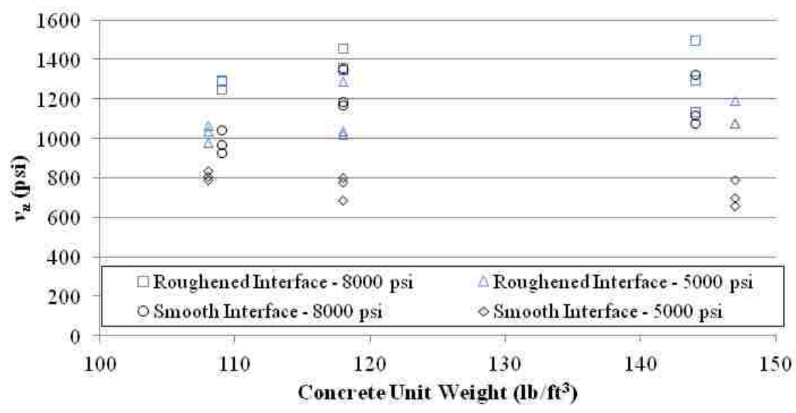
Figure 4.4. Shear strength v_u versus concrete unit weight for all specimens
