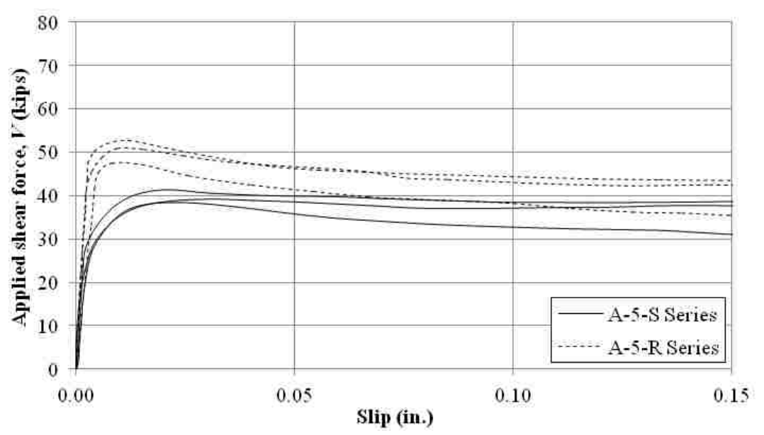
Figure 4.23. Effect of interface roughness on the applied shear force for 5000 psi all-lightweight concrete specimens
