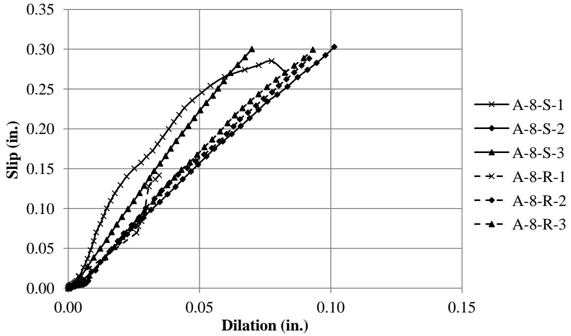
Figure 3.45. Slip vs. dilation for 8000 psi all-lightweight concrete specimens
