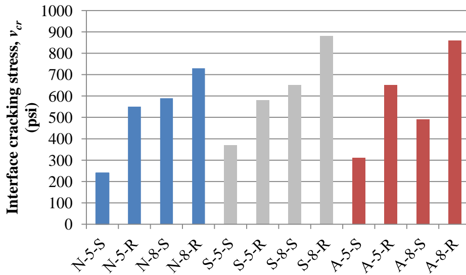
Figure 4.3. Average interface cracking stress, v_{cr} for all series
