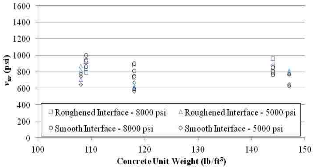
Figure 4.8. Residual shear strength v_{ur} versus concrete unit weight for all specimens
