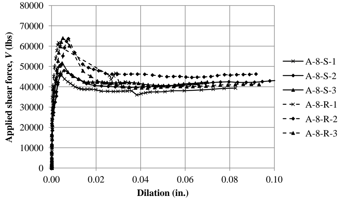
Figure 3.44. Applied shear force vs. dilation relations for 8000 psi all-lightweight concrete specimens
