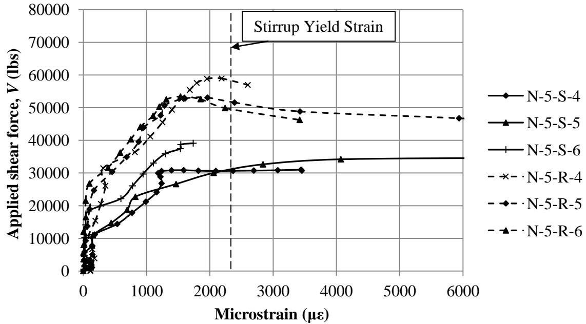
Figure 3.20. Applied shear force vs. interface steel strain for 5000 psi normalweight concrete specimens
