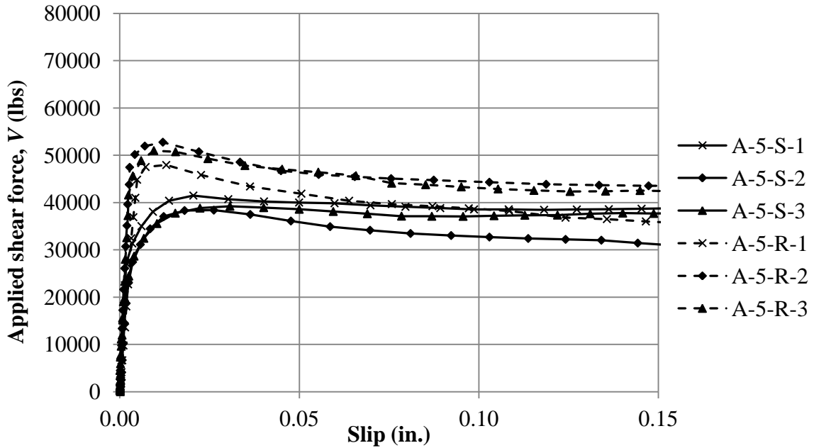
Figure 3.38. Applied shear force vs. slip relations for 5000 psi all-lightweight concrete specimens
