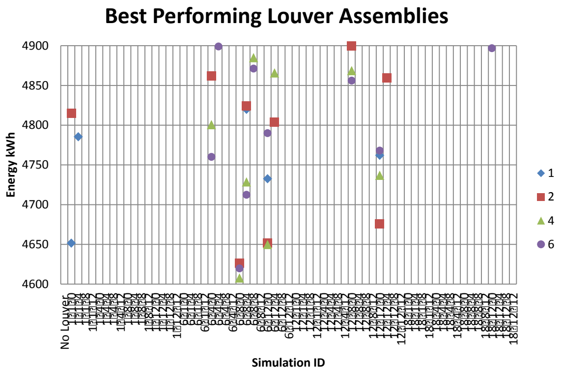
Figure 4.1. Graph of Best Performing Louver Configurations
