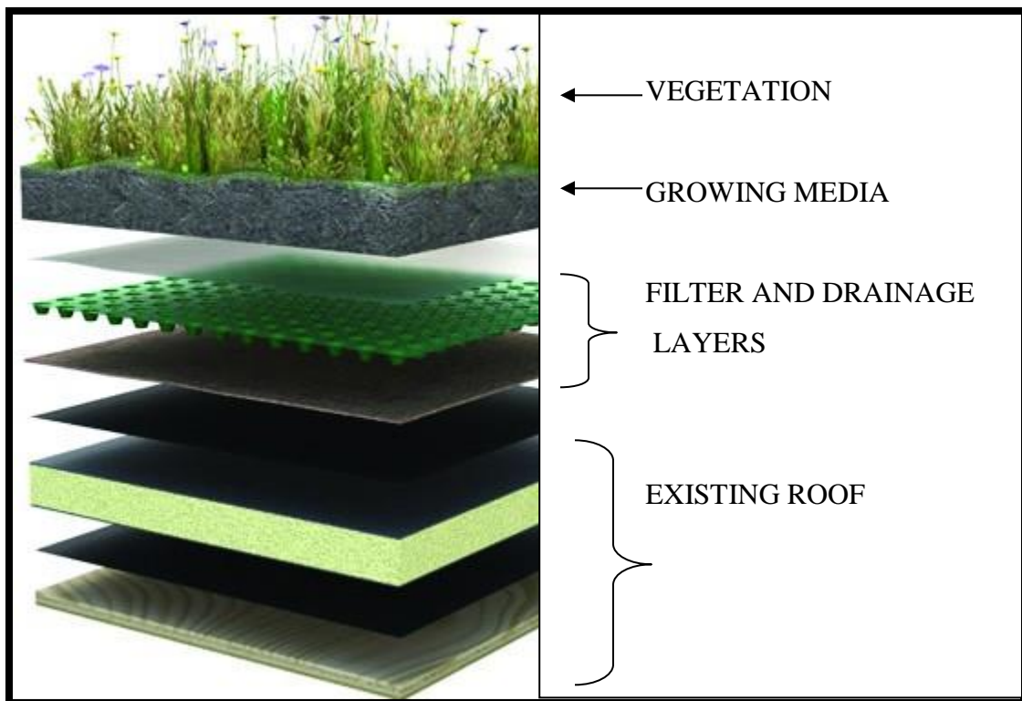
Figure 3.1. Layers of a green roof (Adapted from dgreenworks.org)
