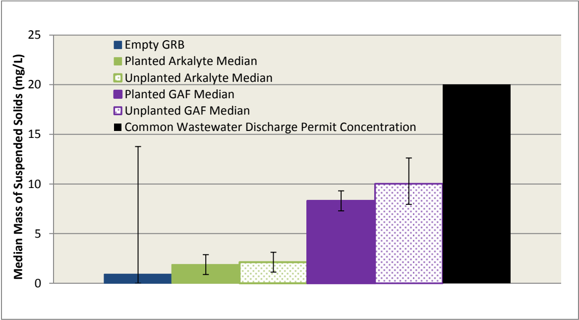
Figure 3.9. Median total suspended solids over the course of the study for each condition tested in Green Roof Blocks™, showing the effectiveness of the filtering layers of both systems.
