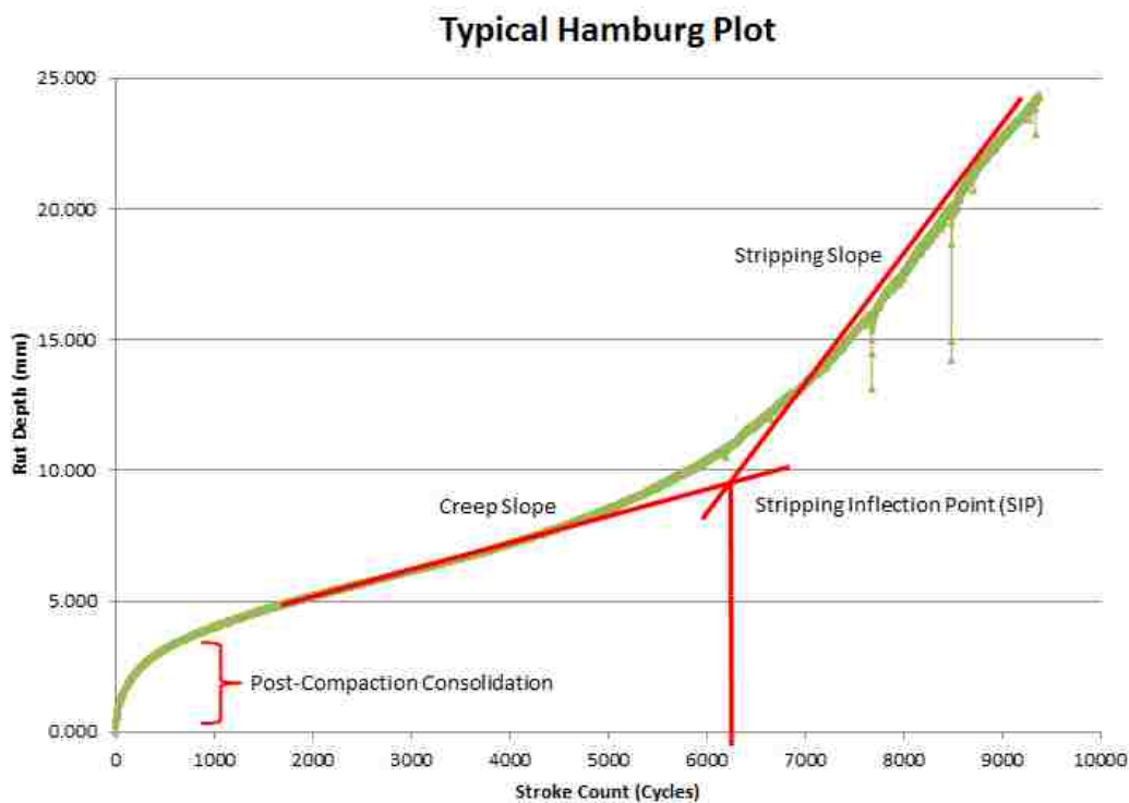
Figure 4.4 - Typical Hamburg Plot with Labels
