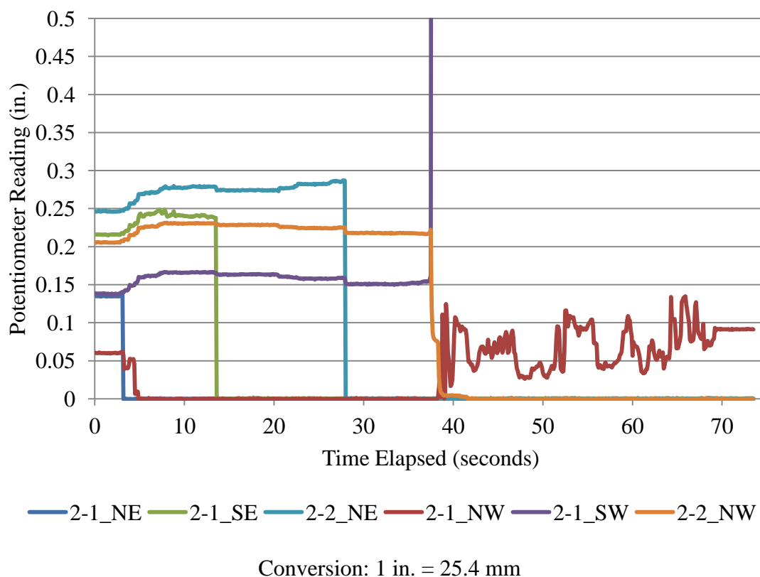
Figure 4.22 – Typical End Slip Plot: C6 Two-Strand Beams Potentiometer Reading vs. Time Elapsed Plot from Synergy
