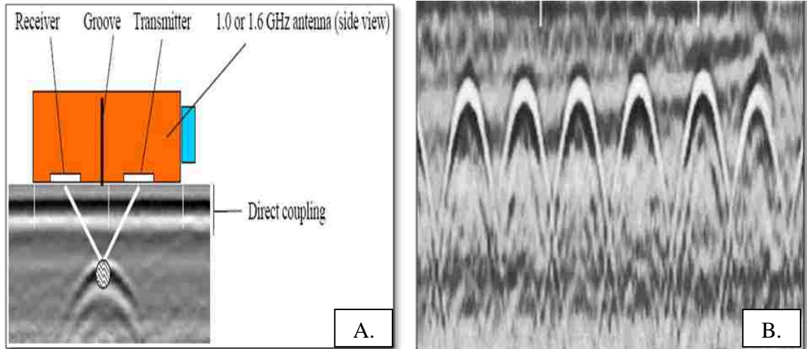
Figure 2.3: Sample images of reinforcing bar (A. GPR image of embedded reinforcing bar, B. Hyperbolic-shaped GPR images of reinforcing bar) (GSSI 2007)
