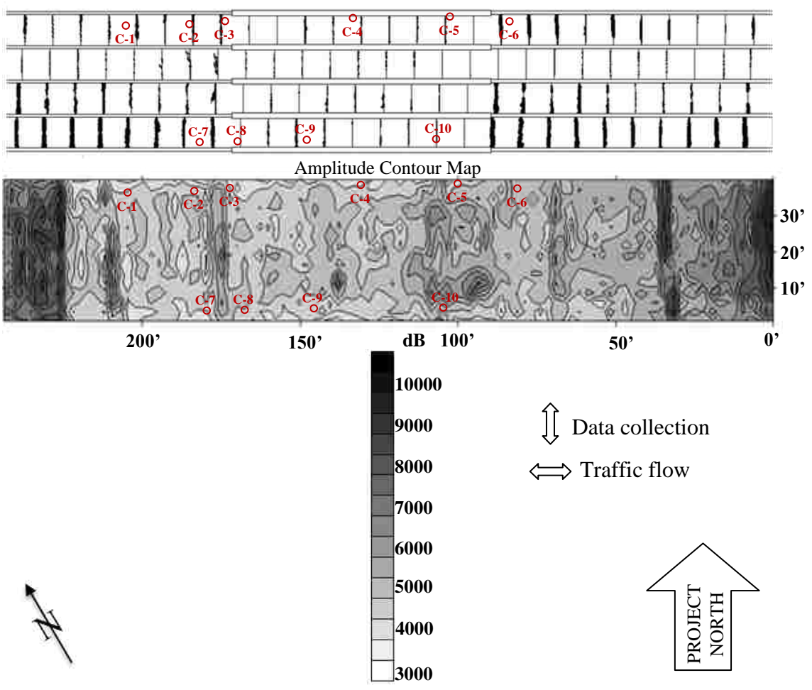
Figure 4.9: Locations of cores with respect to panel locations and GPR deterioration map
