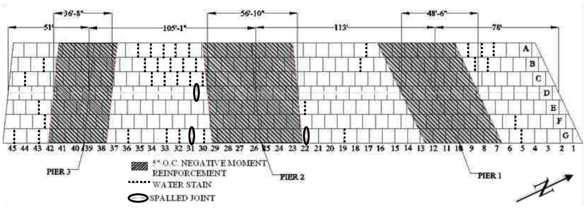
Figure 3.21: Visual inspection results for Bridge A4705
