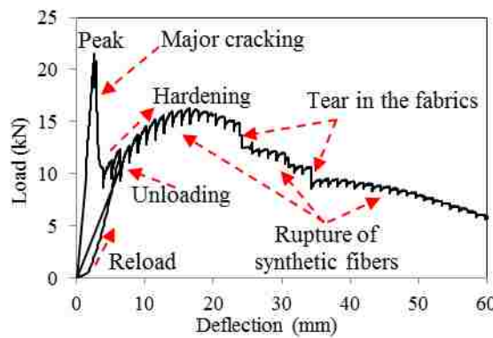
Figure 4.7. Load-deflection curve of Panel P3
