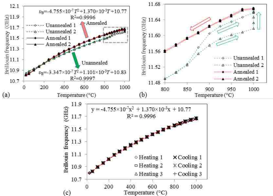
Figure 5.23. Brillouin frequency changes: (a) one cycle of 22–1000 ^\circ\text{C} before and after annealing; (b) one cycle of zoom-in 800–1000 ^\circ\text{C} before and after annealing; (c) three cycles of 22–1000 ^\circ\text{C} after annealing. The Brillouin frequency is denoted by \nu_B
