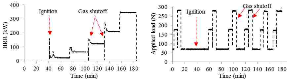
(a) Heat Release Rate (HRR) vs. time
