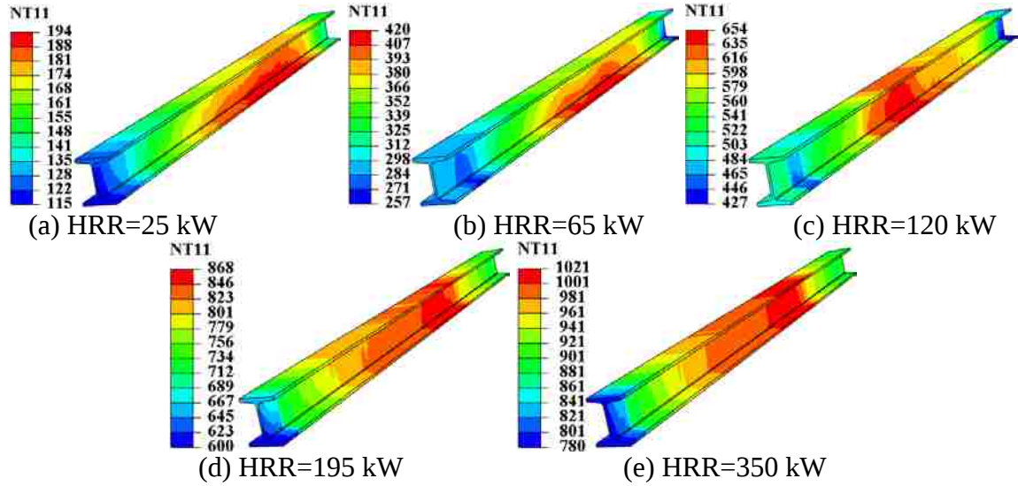
Figure 7.6. Temperature distributions of Beam #2 at various HRRs
