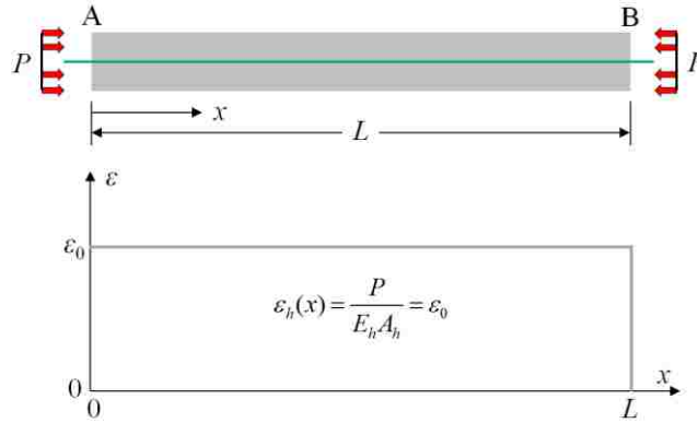
Figure 2.3. Uniaxial tensile test in uniform strain field
