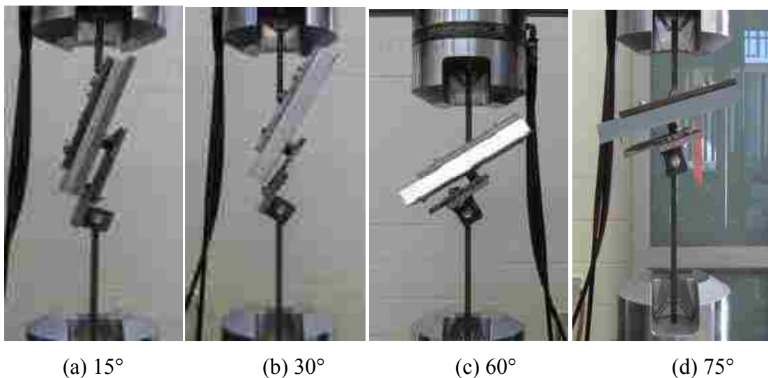
Figure 3.2 Angles of Rotation
