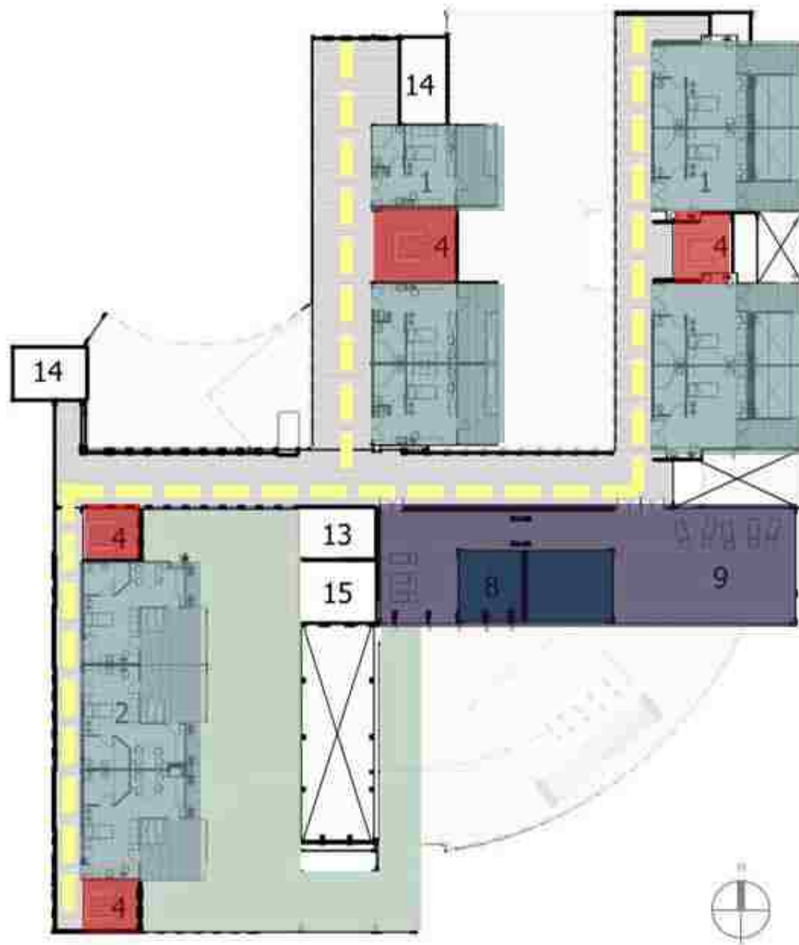
Figure 53: 8 Floor Plan
