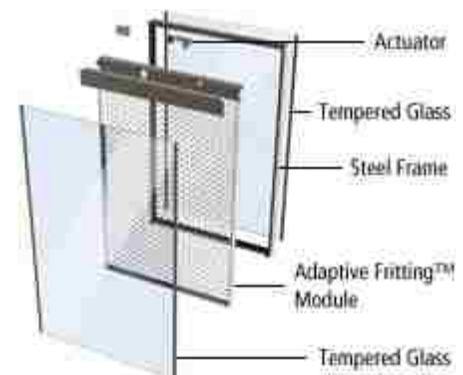
Figure 17 Adaptive Fritting
