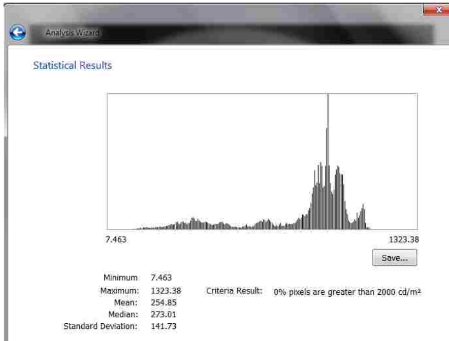
Figure 45 Test Case: Image Luminance Analysis (Results – with blinds control)
