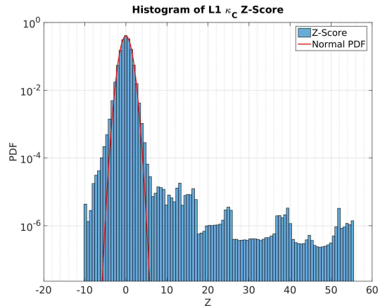
(b) \kappa_C z-score distribution of LLO O2 data.
