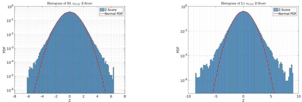
(a) \kappa_{UIM} z-score distribution of LHO O3a data.
