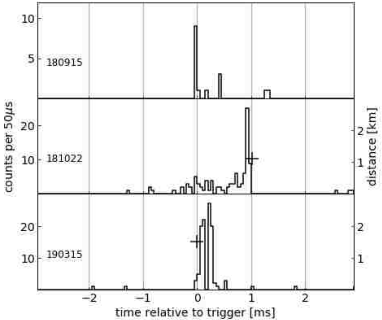
Figure 4.5. Time series of 3 bursts over a 6 ms window binned in 50 \mu s bins. The lightning radio signals are represented by the +.
