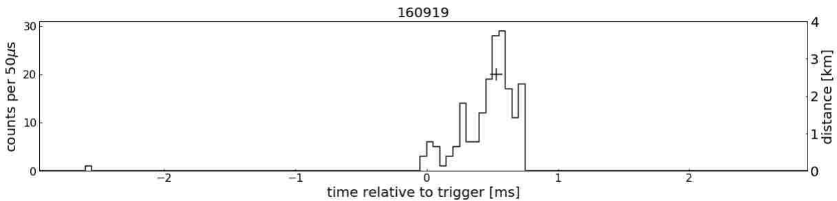
Figure 4.3. Time series over a 6 ms window binned in 50 \mu\text{s} bins for the Puerto Rico event at 18:09:33 UTC on 19 September 2016, summed over all BGO in four boxes. The lightning radio signal is represented by the +.
