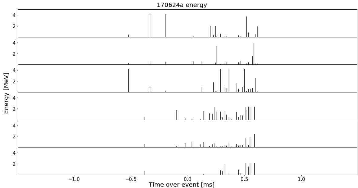
Figure 4.8. Individual BGO energy readings from event at LSU at 19:34:50 UTC on 24 June 2017. Peak energy seen up to 4 MeV over \sim 1 ms.
