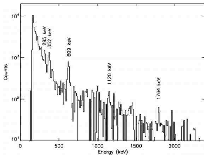
Figure 5.1. High resolution spectrum observed by TETRA-I showing the emission lines of radon daughters produced during a 4 hr rainfall event (Ringuette et al., 2013).
