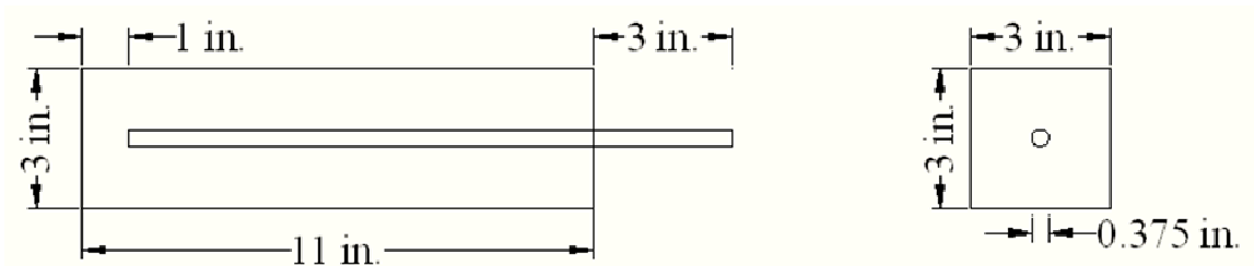
Figure 3.2. Specimens with side edge distance of 1.5 in.
