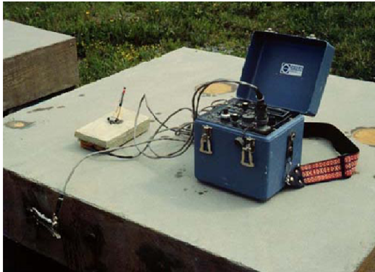
Figure 2.6. 3LP device (Zemajtis 1998)
